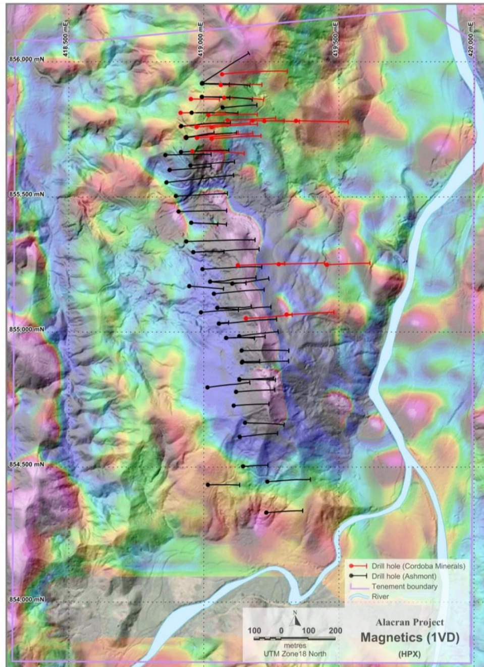
Figure 9-4: 2016 El Alacrán First Vertical Derivative Ground Magnetic Survey
