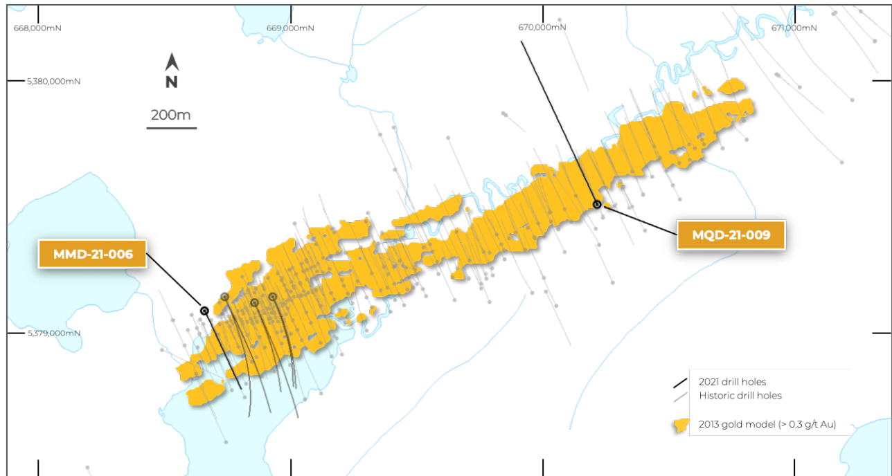
Figure 4: Drill plan showing the 2021 drill holes relative to the 2013 resource model and historic drill hole location
