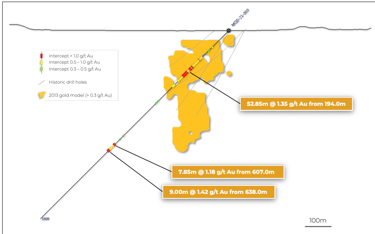
Figure 3: Drill section through MQD-21-009 (hole not yet surveyed) showing mineralized intercepts relative to the 2013 grade model
