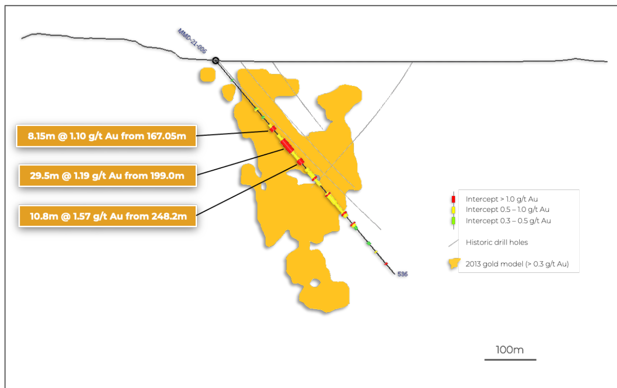
Figure 2: Drill section through MMD-21-006 (hole not yet surveyed) showing mineralized intercepts relative to the 2013 grade model
