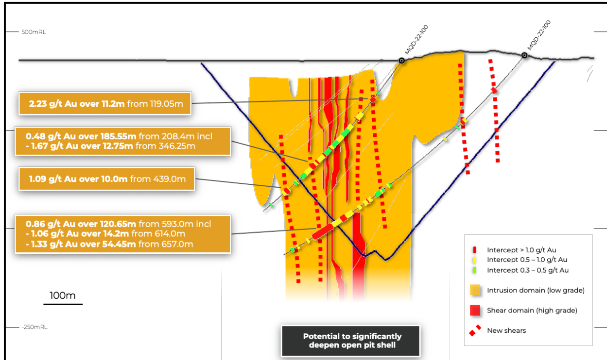
Figure 2: Drill section through MQD-22-100 and -104 relative to the current Mineral Resource and highlighting the additional shears and potential to significantly deepen the open pit shell
