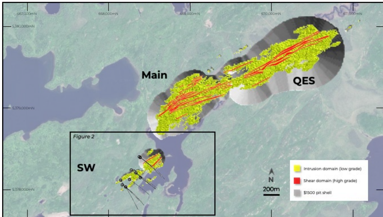
Figure 1: Location of drill holes in this release relative to the November 2022 MRE and $1,500 open pit shell constraint.
