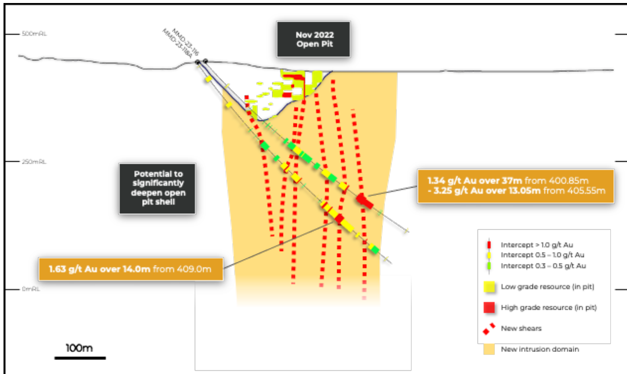
Figure 3: Drill section through holes MMD-23-116 and -118A showing the significant expansion of the mineralized model beneath the November 2022 MRE and $1,500 open pit shell constraint, which should add to mineral resources in the May 2023 MRE.
