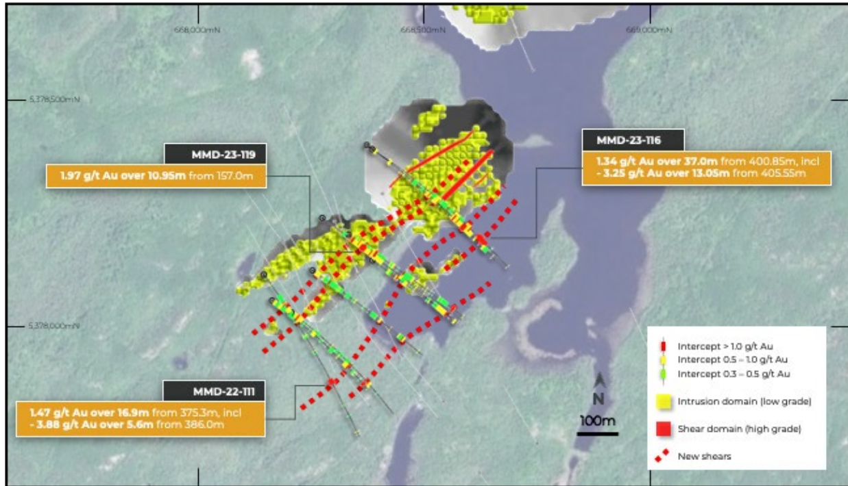
Figure 2: close up of Southwest Zone with significant intercepts relative to the November 2022 MRE and $1,500 open pit shell constraint.
