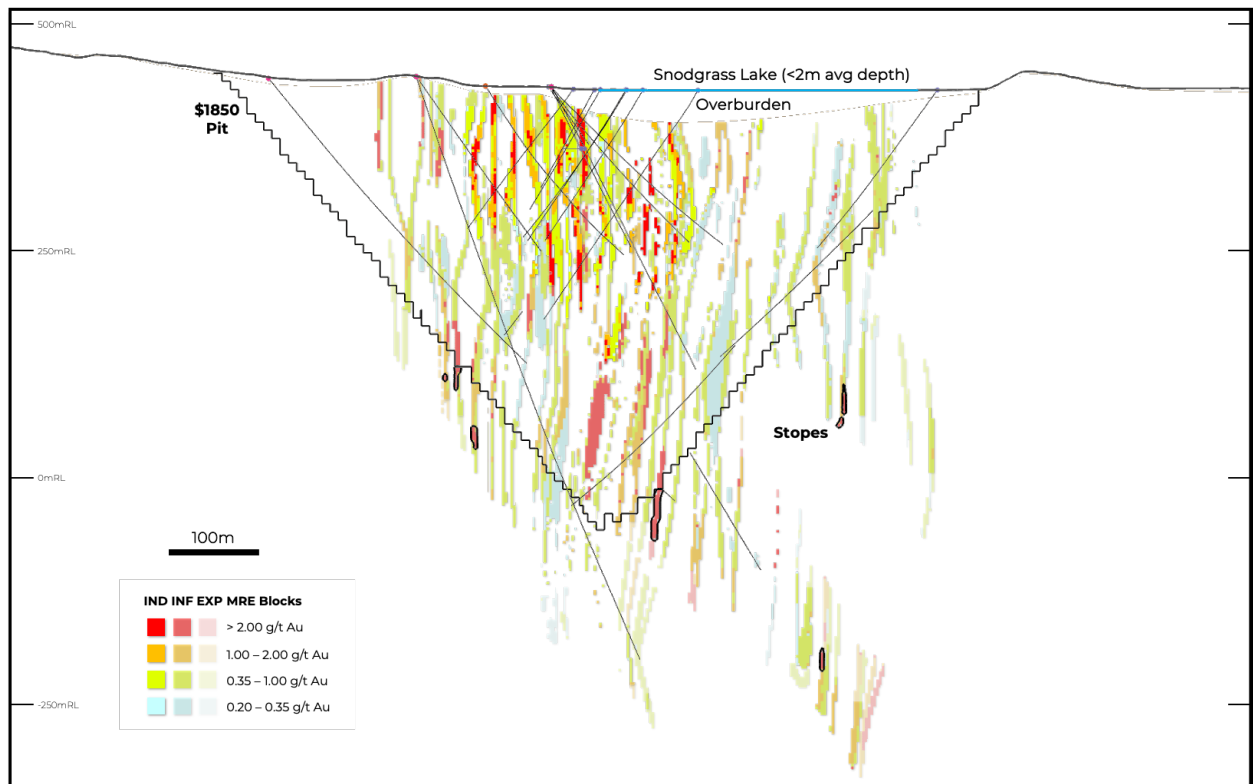
Figure 4: Cross section through the Moss Main Zone showing grade model, $1850 open pit shell and modelled stopes
