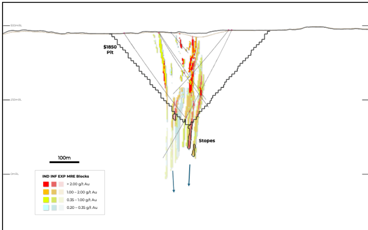
Figure 7: Cross section through East Coldstream showing grade model, $1,850 open pit shell and modelled stopes
