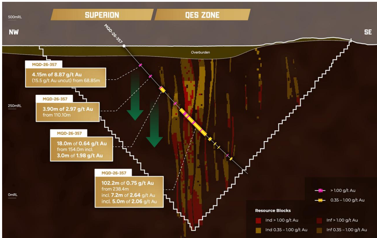
Figure 2: Shows a typical section through drill hole MQD-26-357 with reported intersections relative to the current resource block model
