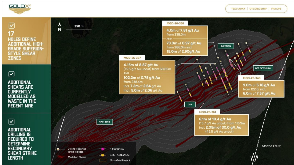
Figure 1: Shows the location of the drill holes across the marginal shears in the Superior Zone
