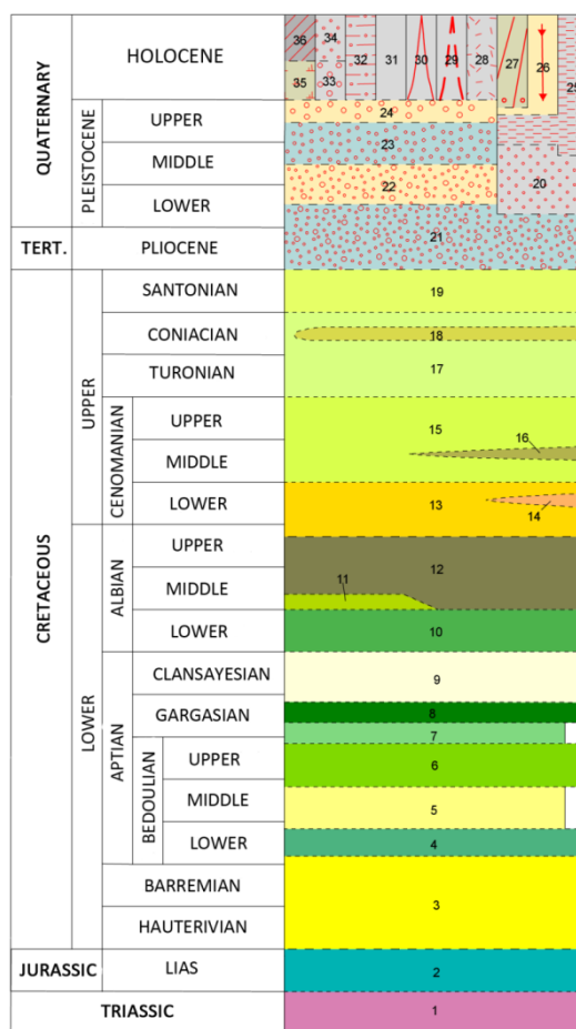
Figure 22: Stratigraphic Column for Santillana Syncline area. (IGME) (Magna N° 34, series 1: 25,000)
