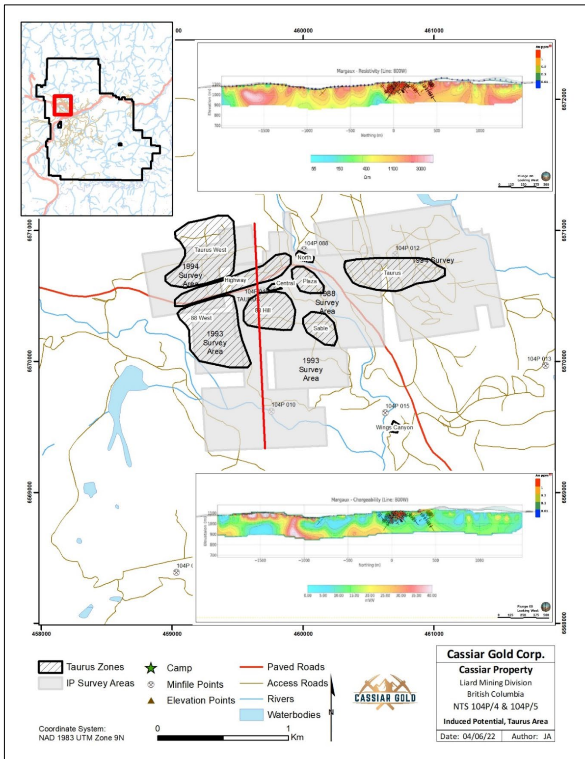
Figure 6-4 Cassiar Gold Property Induced Polarization, Taurus Area
