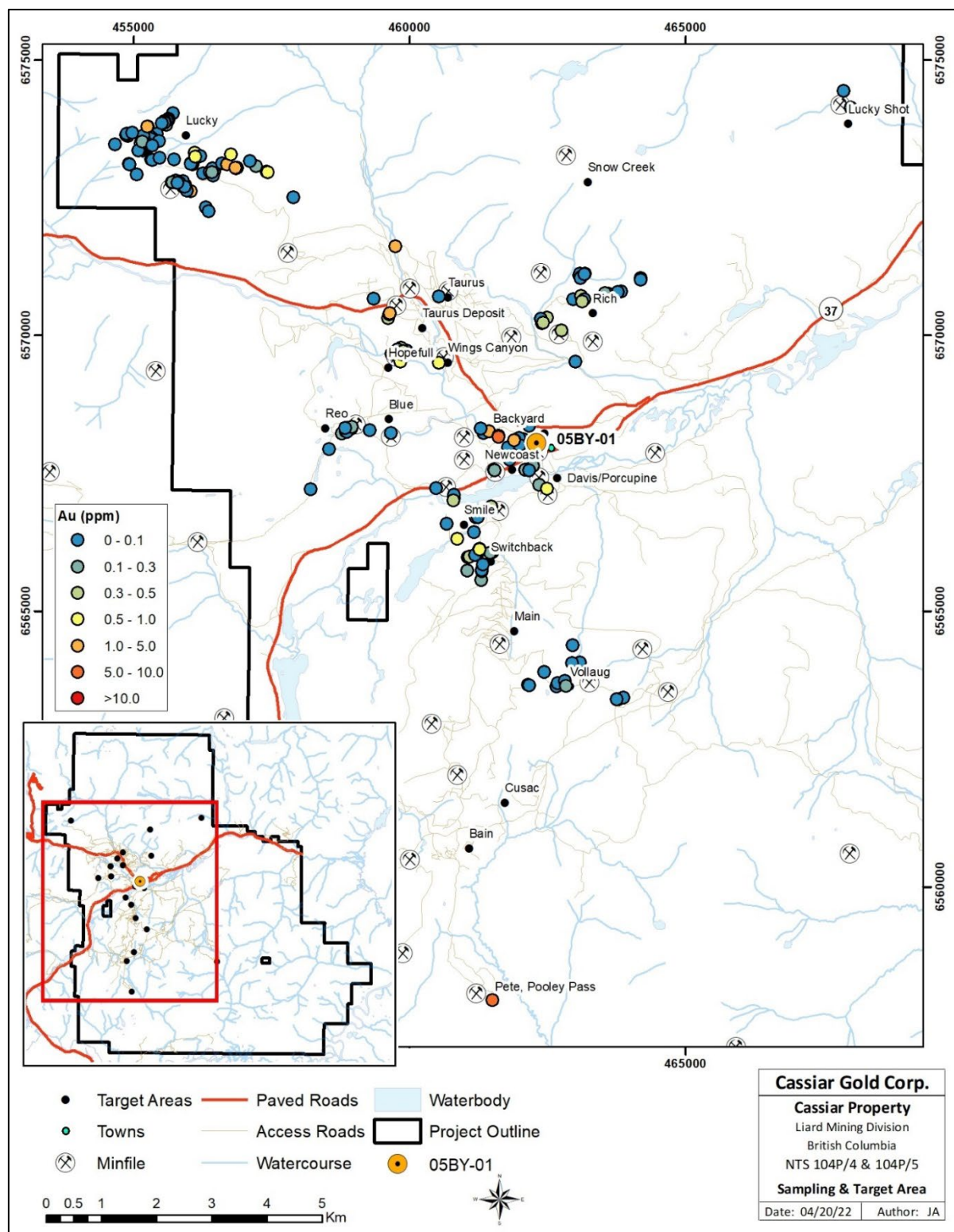
Figure 9-1 Rock and Chip Sample locations 2019
