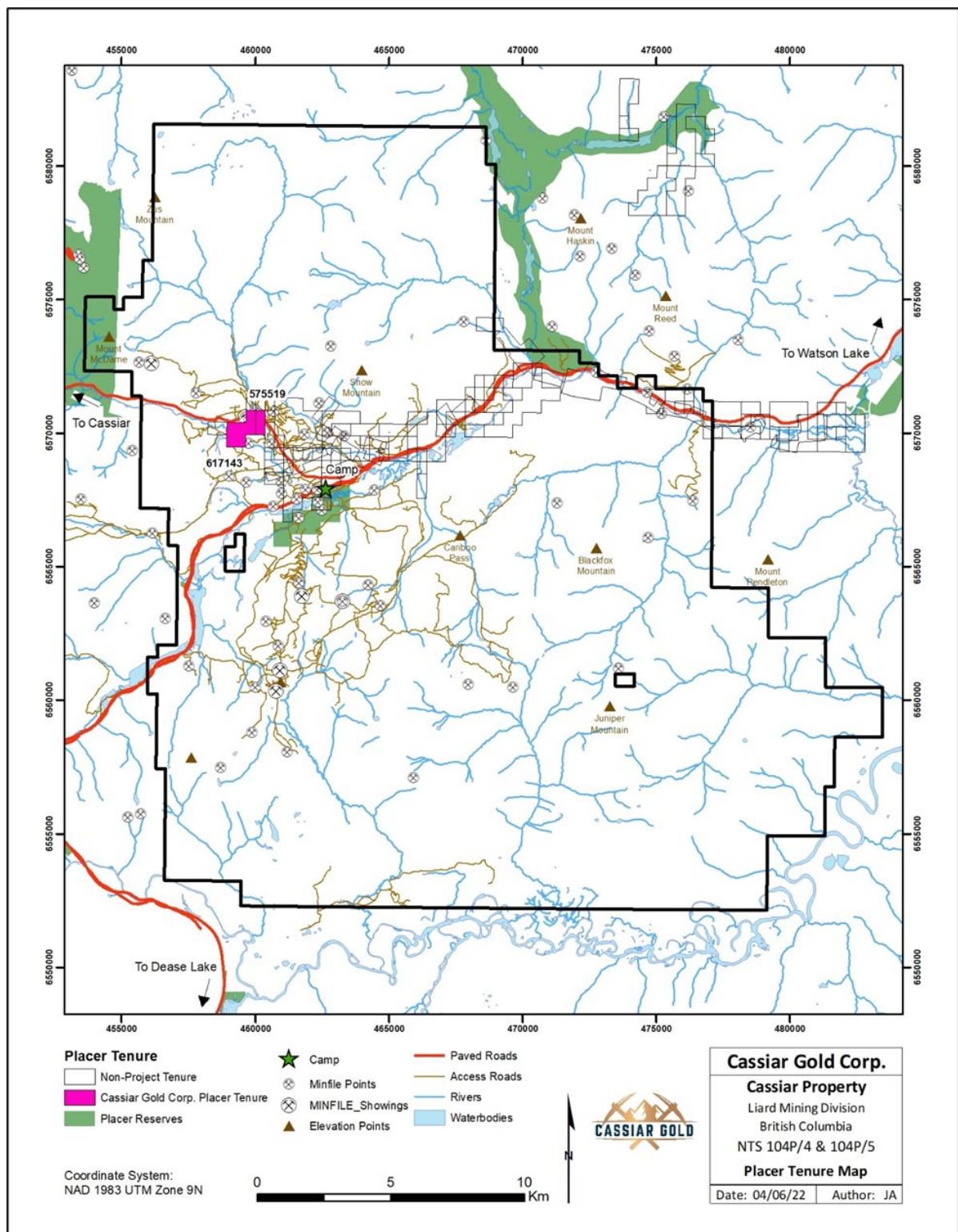
Figure 4-5 Cassiar Gold Property Placer Tenure Map
