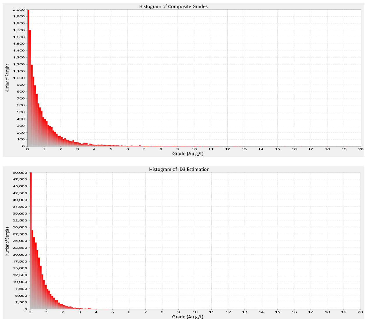
Figure 14-11 Histograms of all zones (Top – composites, Bottom – block model results)
