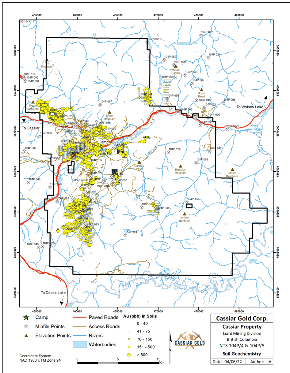
Figure 6-2 Cassiar Gold Property Soil Geochemistry
