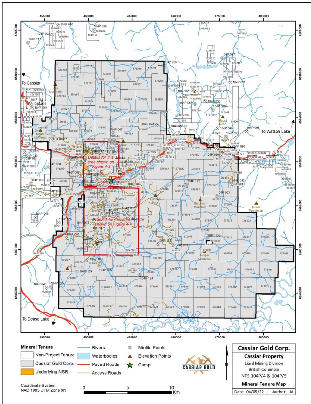
Figure 4-2 Cassiar Gold Property Mineral Tenure Map
