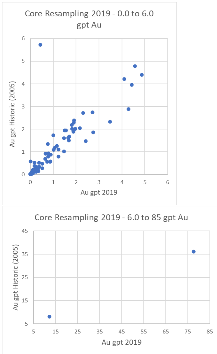
Figure 9-2 Core Resampling Comparison: 0.0 to 6.0 g/t Au and 6.0 to 85 g/t Au
