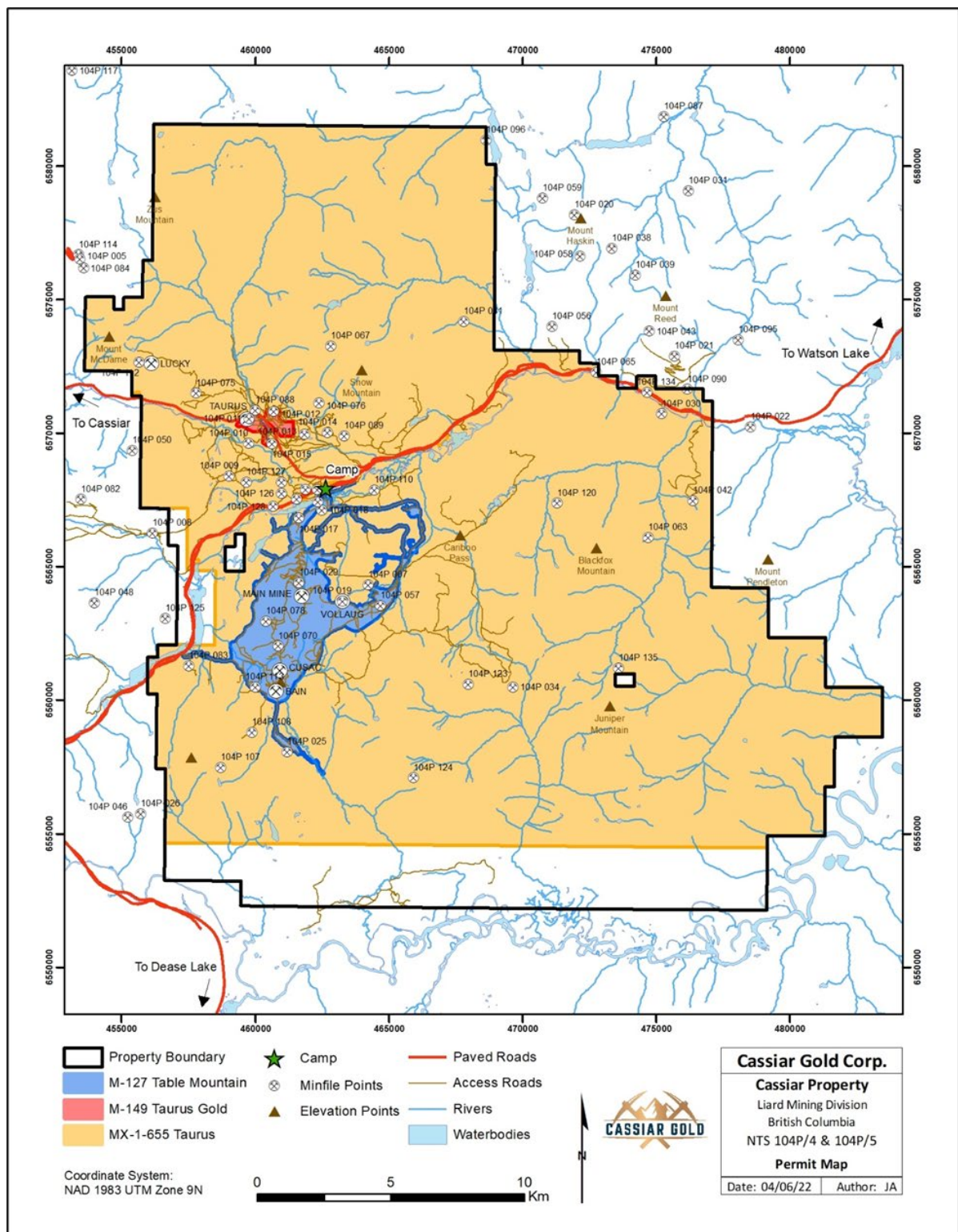
Figure 4-8 Cassiar Gold Property Permit Map
