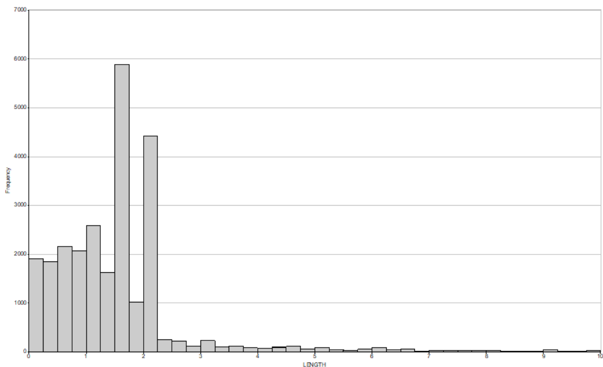
Figure 14-5 Drill hole Histogram for Sample Length
