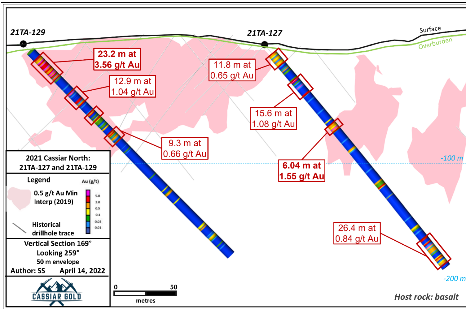
Figure 10-6 Taurus/Hill 88 Drill Section
