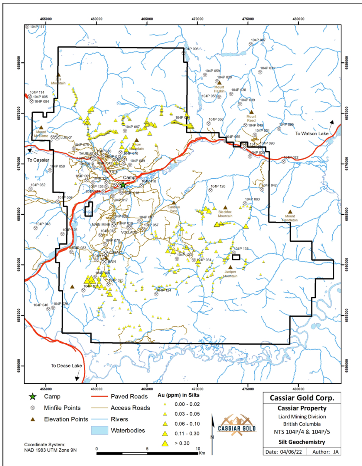
Figure 6-3 Cassiar Gold Property Silt Geochemistry
