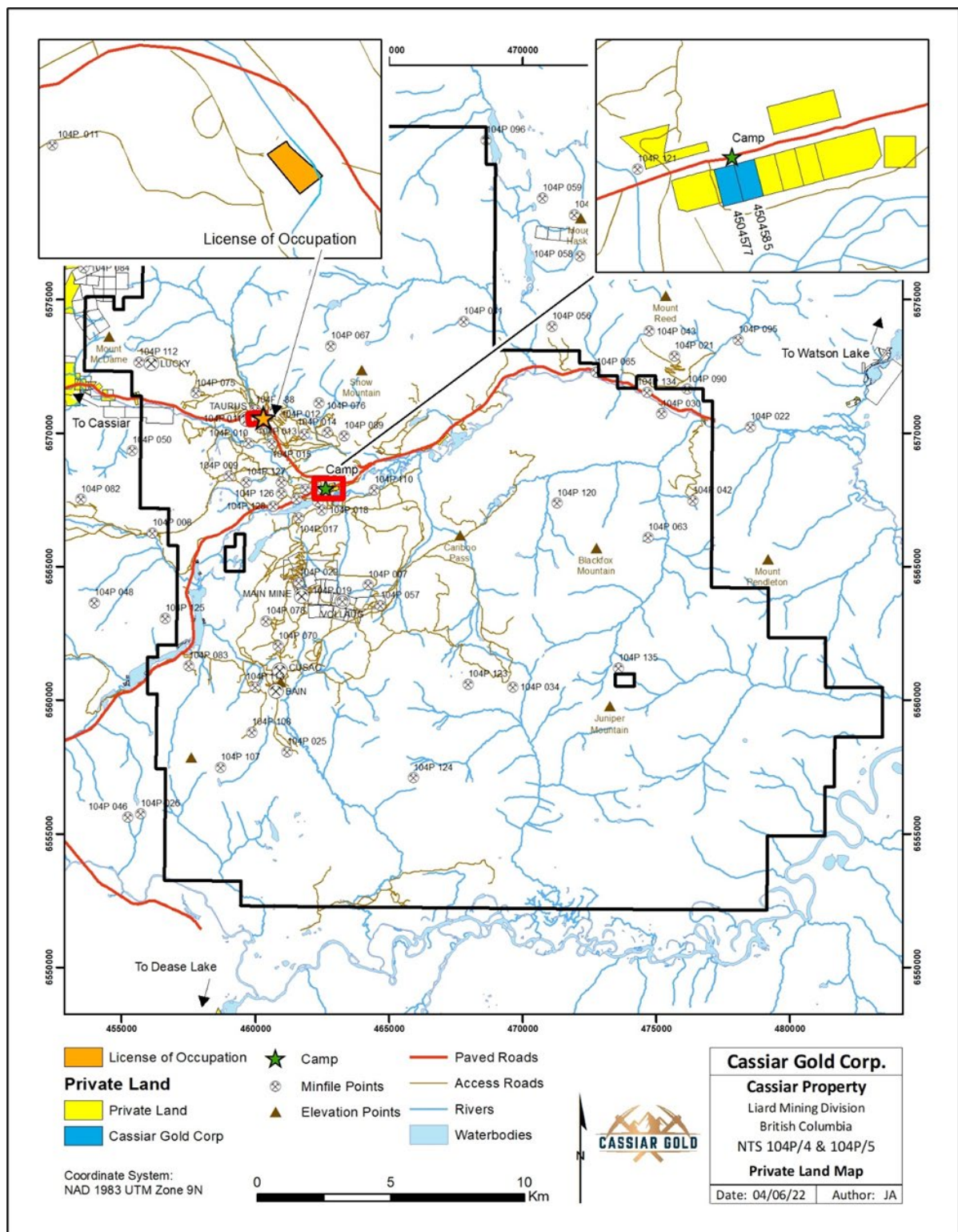
Figure 4-7 Cassiar Gold Property Surface Tenure Map
