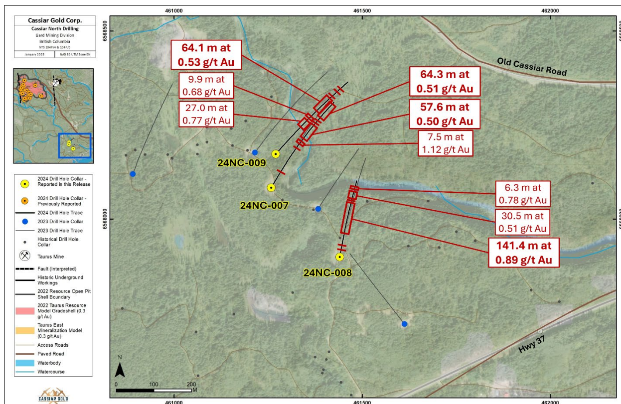
Figure 3. Plan view map of 2024 drill holes reported in this news release. The map location is shown in Figure 1. The vertical projection of mineralized intercepts reported in this release are included for reference.
