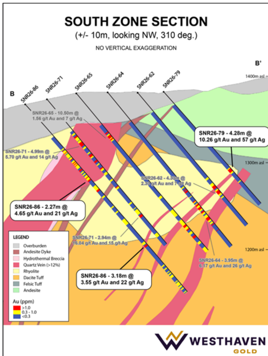
Figure 3 – South Zone Cross Section B-B'
