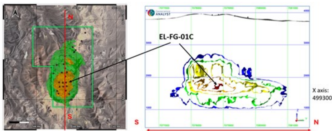
Figure 4: Combined plan and cross-sectional views of the Cohen (2011) porphyry footprint modelling results based on multi-element rock geochemistry.
