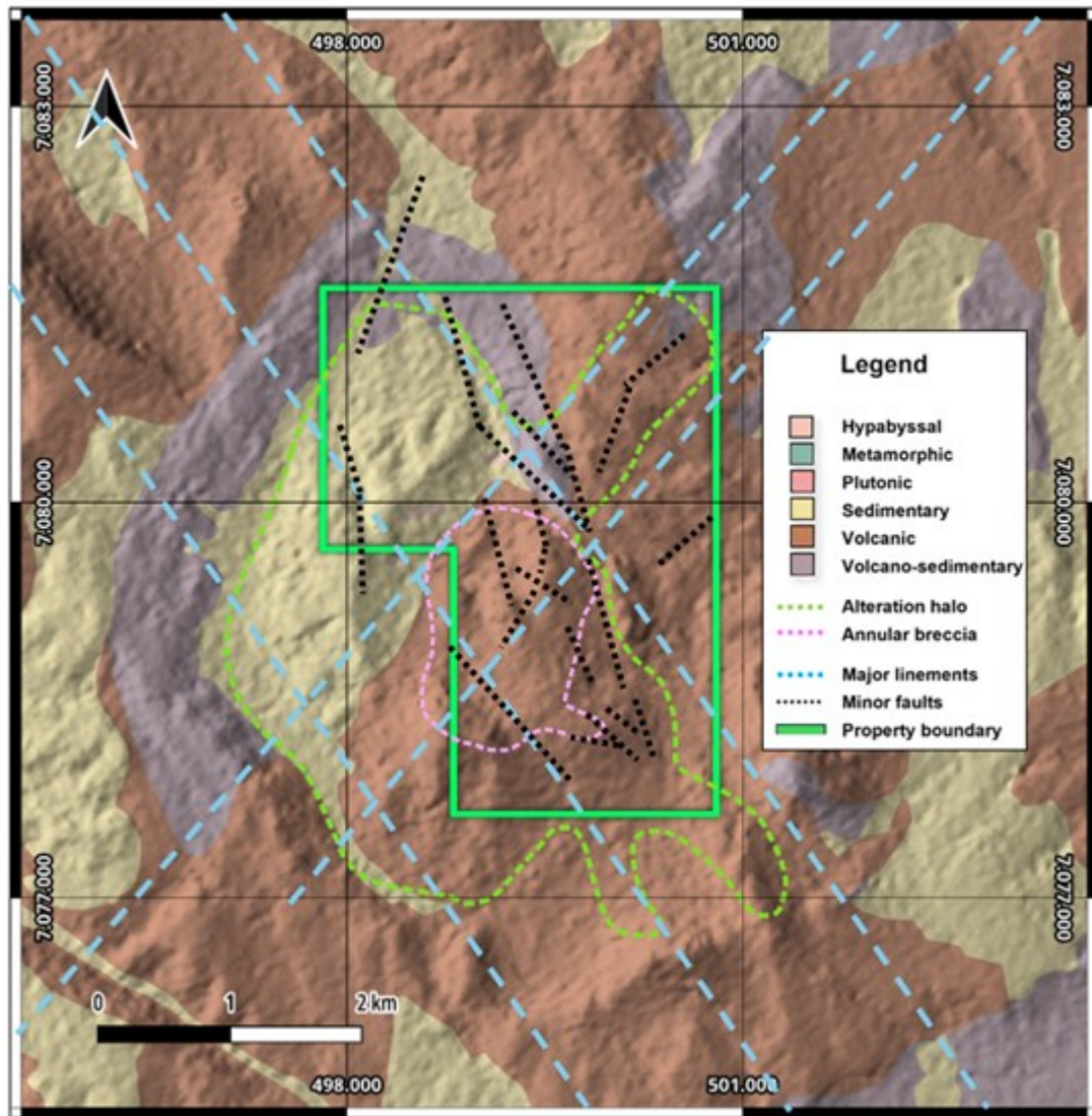
Figure 2: Elvira Project concession boundary and simplified geological map.
