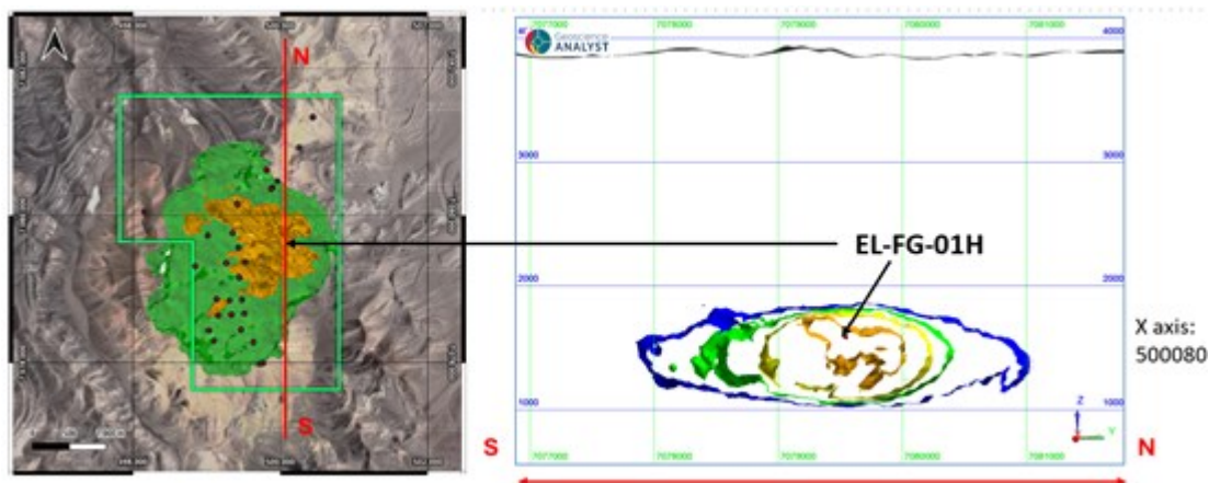
Figure 5: Combined plan and cross-sectional views of the Halley et al. (2015) porphyry footprint modelling results based on multi-element rock geochemistry.
