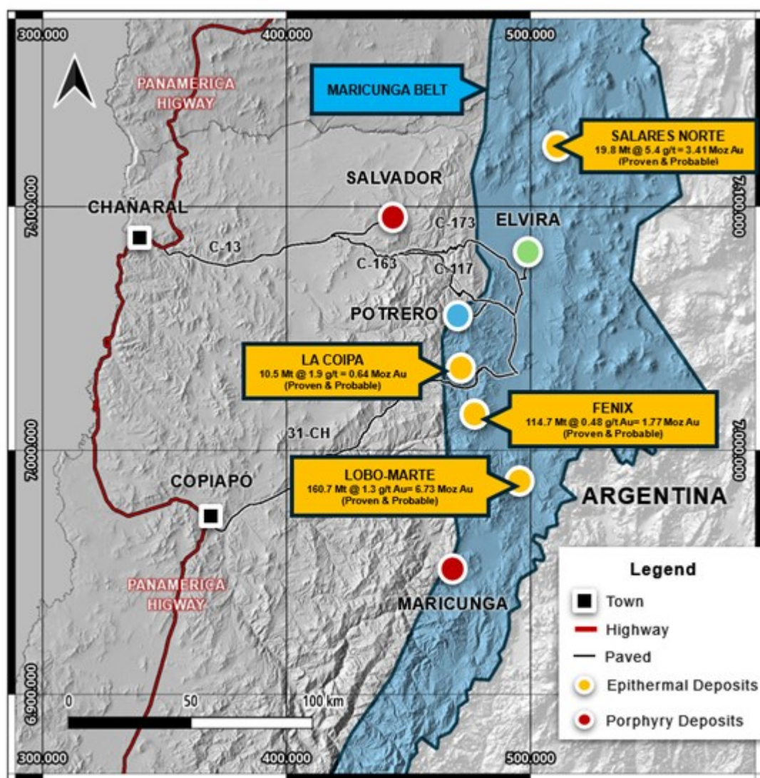
Figure 1: Regional location map of the Elvira Project, Maricunga Belt, Chile*.
