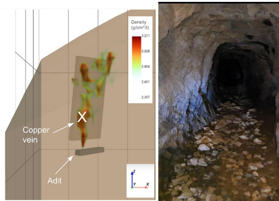
ORE Modelled 3d density prediction (left) and Anvil Adit (right) in Idaho
