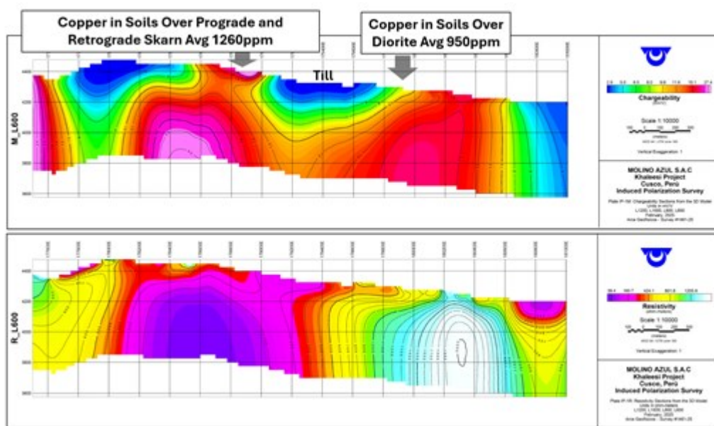
Figure 3: Vertical section chargeability (top) and resistivity (bottom) plot of 2025 IP survey line 600N (shown in Figure 2), looking to the north. The chargeability and resistivity anomalies have never been drill tested by C3 Metals or historically and correlate well with surface copper geochemistry.
