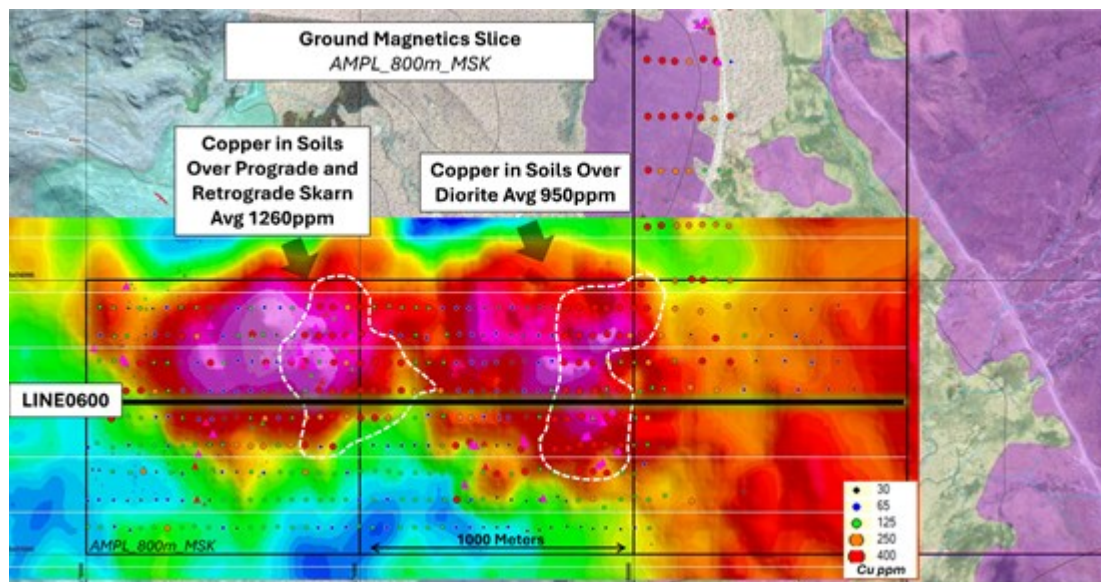
Figure 2: MVI Magnetic Inversion: Amplitude of Magnetization, depth slice 800m showing two large magnetic anomalies. The geophysical anomalies remain open along-strike to the east.
