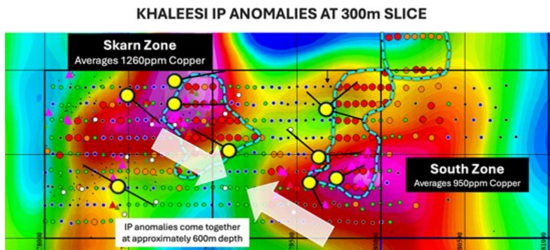
Figure 1: Plan view map of IP chargeability anomalies at 300m depth showing drill collar and hole locations for the initial Khaleesi 14-hole, 6,300m drill program. Note the locations of the strong copper in soil geochemical anomalies over the IP chargeability anomalies. The two IP chargeability anomalies come together at approximately 600m depth.
