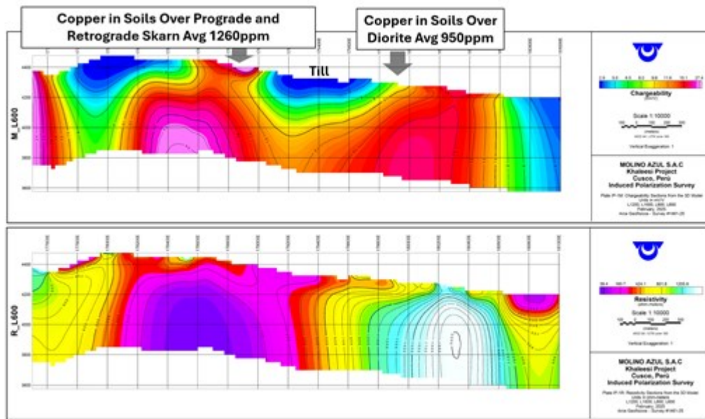
Figure 4: Vertical section chargeability (top) and resistivity (bottom) plot of 2025 IP survey line 600N (shown in Figure 3), looking to the north. The chargeability and resistivity anomalies correlate well with surface copper geochemistry.
