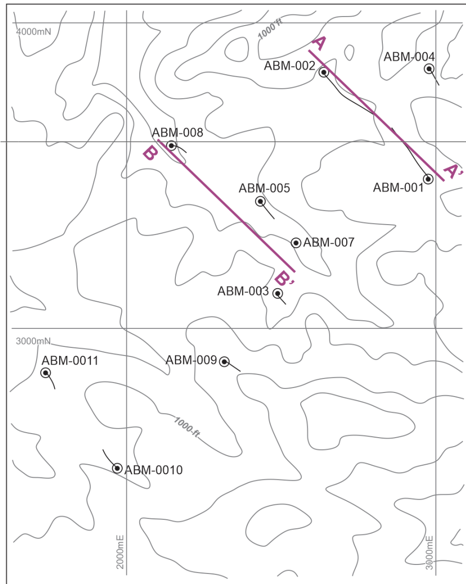
Figure 1: Location of drill collars and drill traces, Mountain Zinc-Copper Project, Virginia. Cross sections traces A-A' and B-B'. Local grid in metres.
