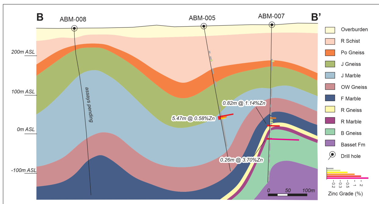
Figure 3: Cross section B-B' with significant zinc intercepts, Mountain Zinc-Copper Project, Virginia. View looking northeast.
