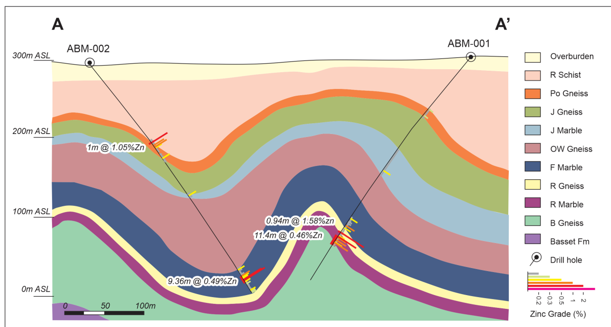
Figure 2: Cross section A-A' with significant zinc intercepts, Mountain Zinc-Copper Project, Virginia. View looking northeast.
