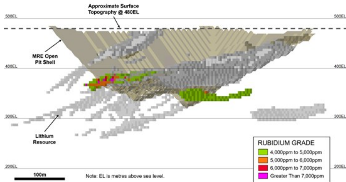
Figure 2: Rubidium MRE isometric section view looking southwest with rubidium grades.
