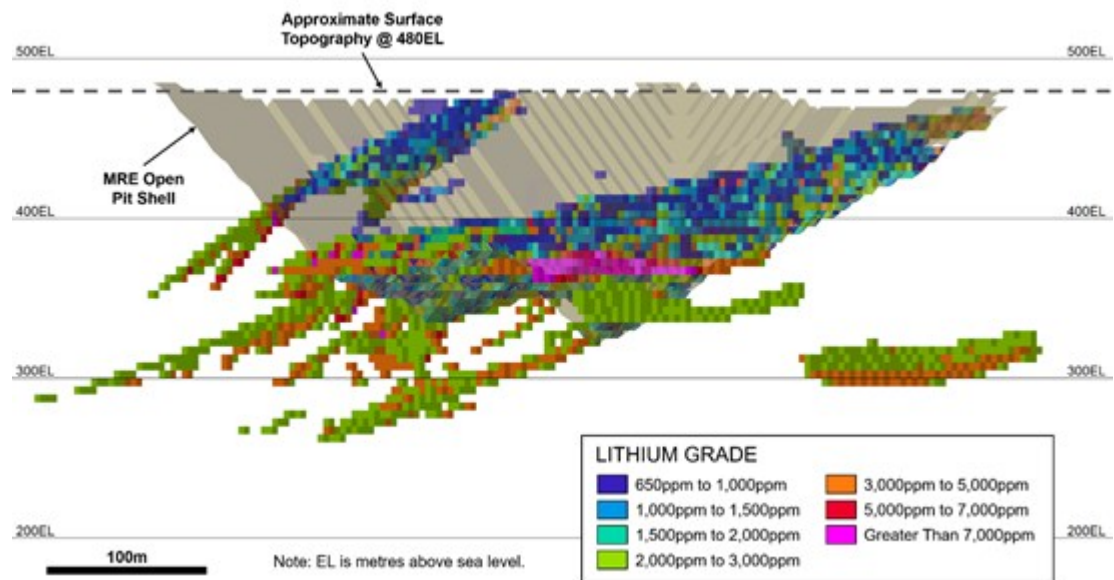
Figure 1: Lithium MRE isometric section view looking southwest with lithium grades.
