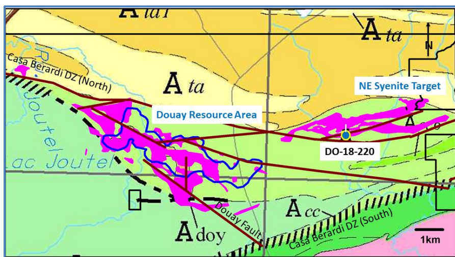
Figure 1: Magnitude of NE Syenite Target vs Douay Resource Area. Note position of initial hole DO-18-220. Geological base map shows location of both syenitic intrusive complexes within Casa Berardi Tectonic Zone.
