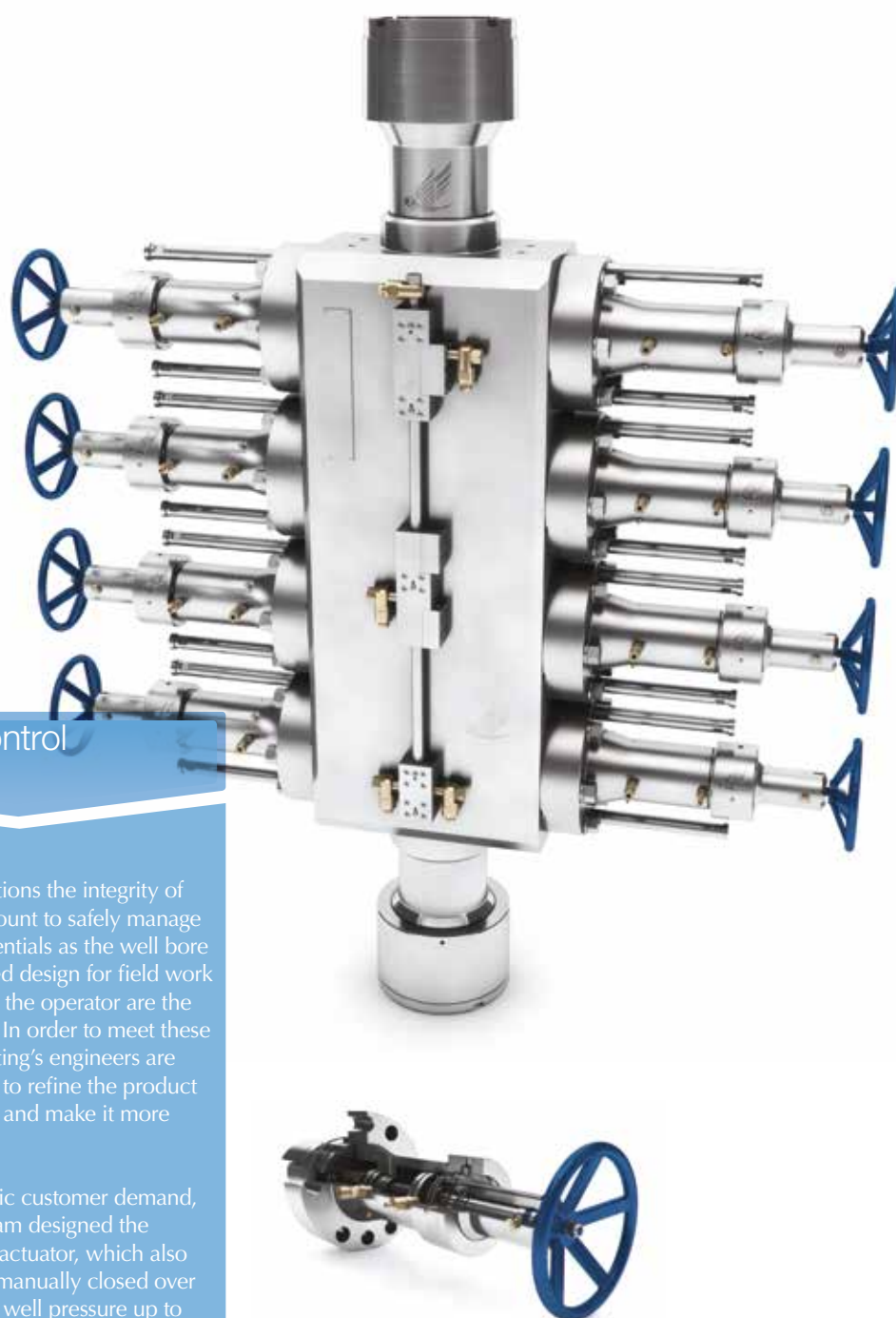
Eziclose quad valve customised for optional manual operation.
