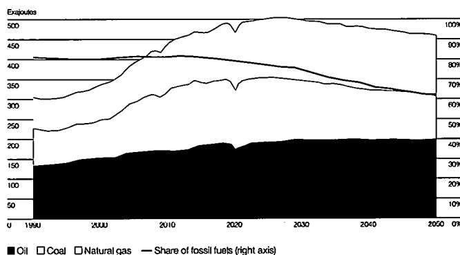
IEA projected fossil fuel demand: 1990-2050
