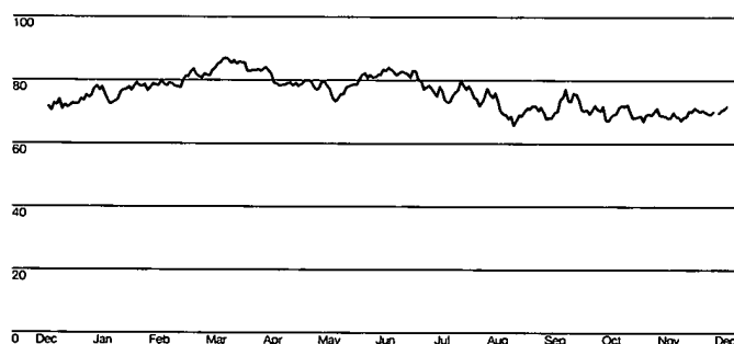
WTI crude oil price 2024 $ per barrel
