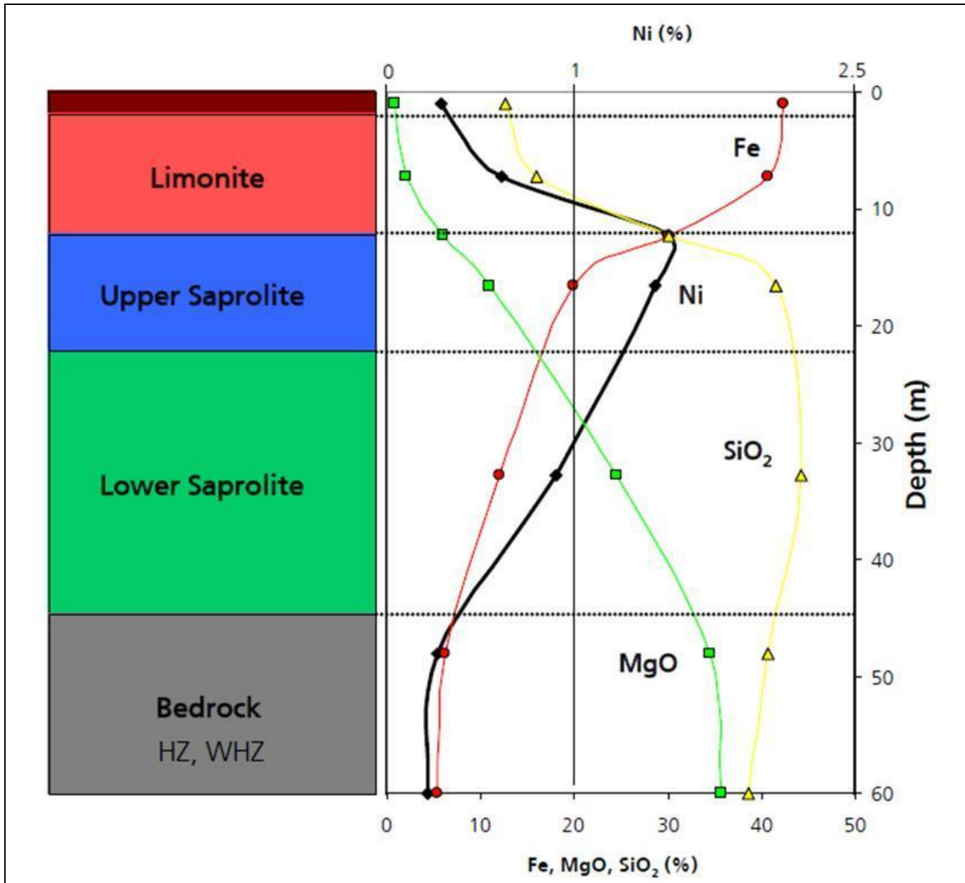
Figure 8.1 Chemical trends in schematic nickel laterite profile
