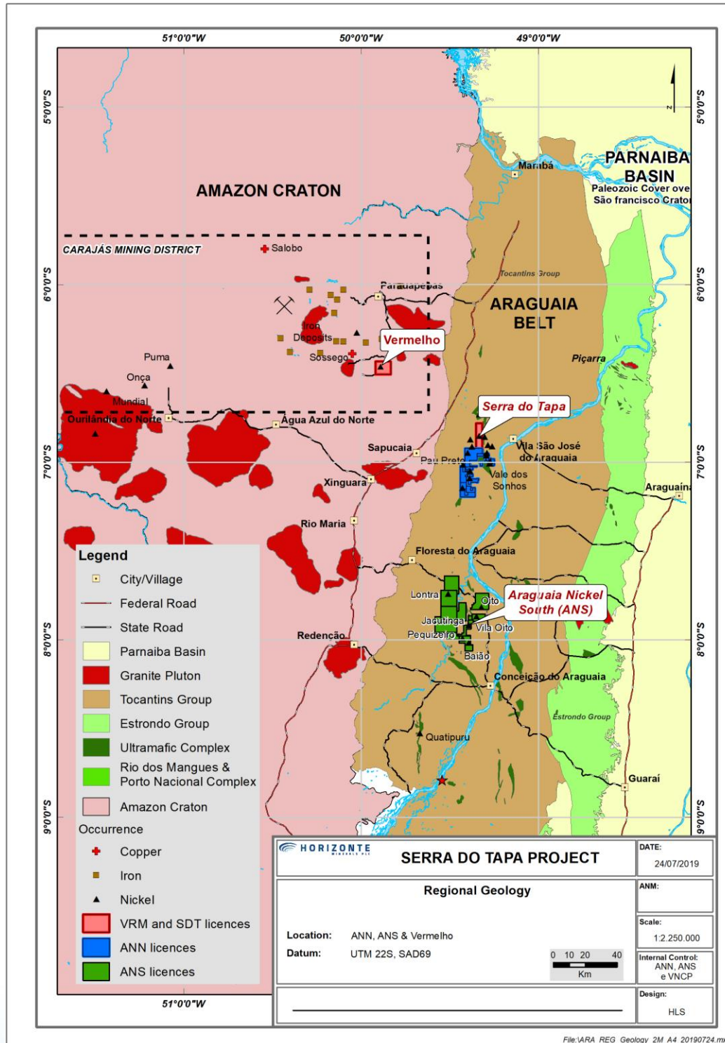
Figure 7.1 Regional geologic setting
