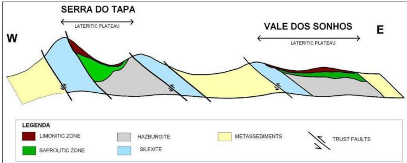
Figure 7.3 Schematic vertical section of SDT and VDS deposits
