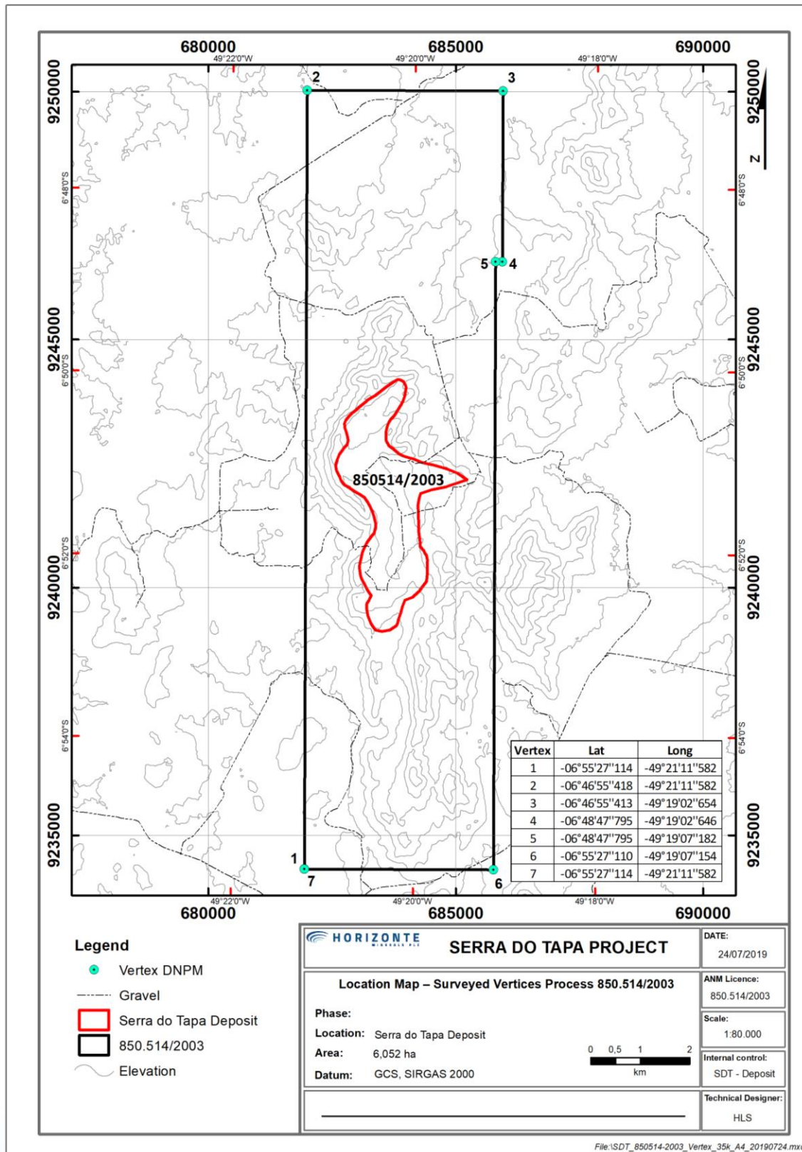
Figure 4.2 SDT licence – surveyed vertices
