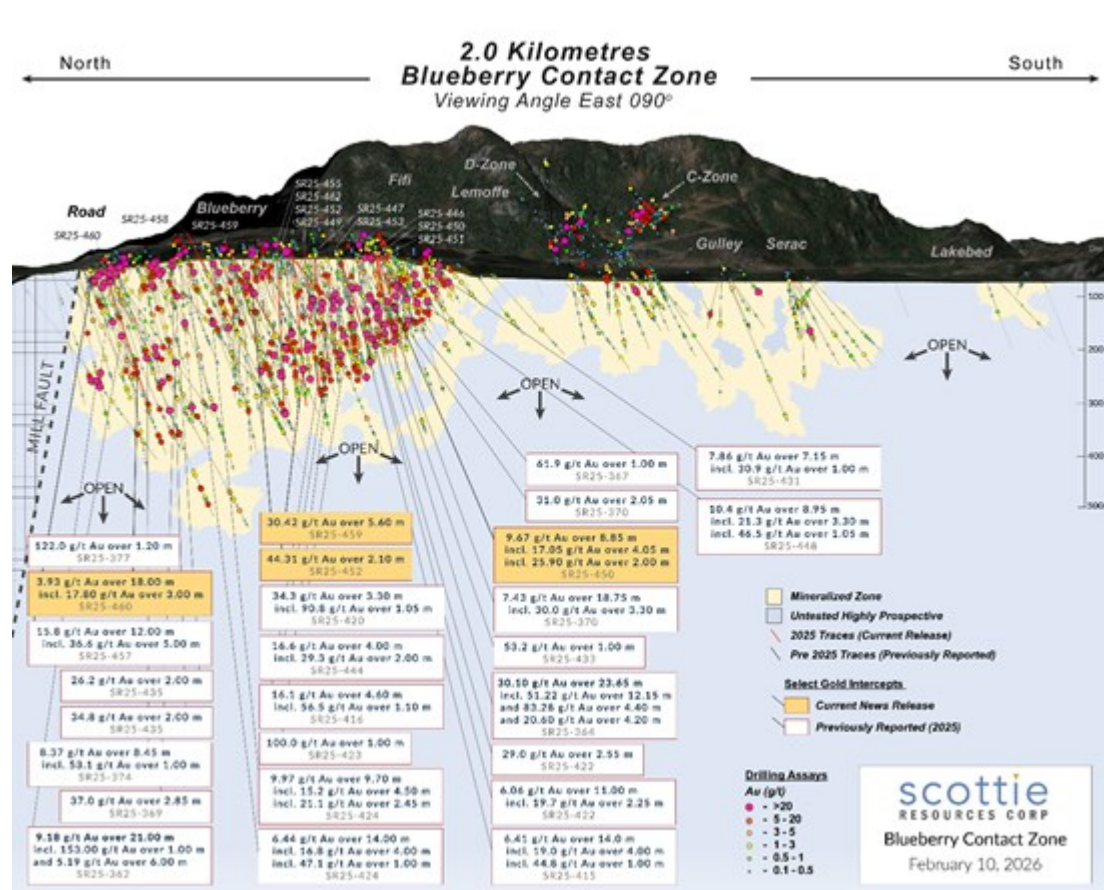
Figure 1: Segmented vertical long section of the Blueberry Contact Zone illustrating the distribution and status of drilled targets from the 2025 season and the reported results thus far, relative to intercepts from previous drilling campaigns.
