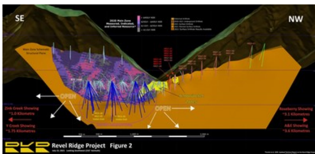
Figure 2. RRMZ Longitudinal Section (CNW Group/Rokmaster Resources Corp.)
