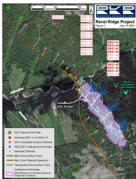
Figure 1. Plan Map 2021 Surface Drilling (CNW Group/Rokmaster Resources Corp.)
