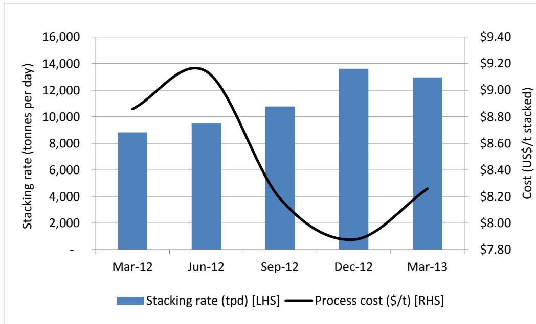
Figure 9 – Process cost per tonne stacked
