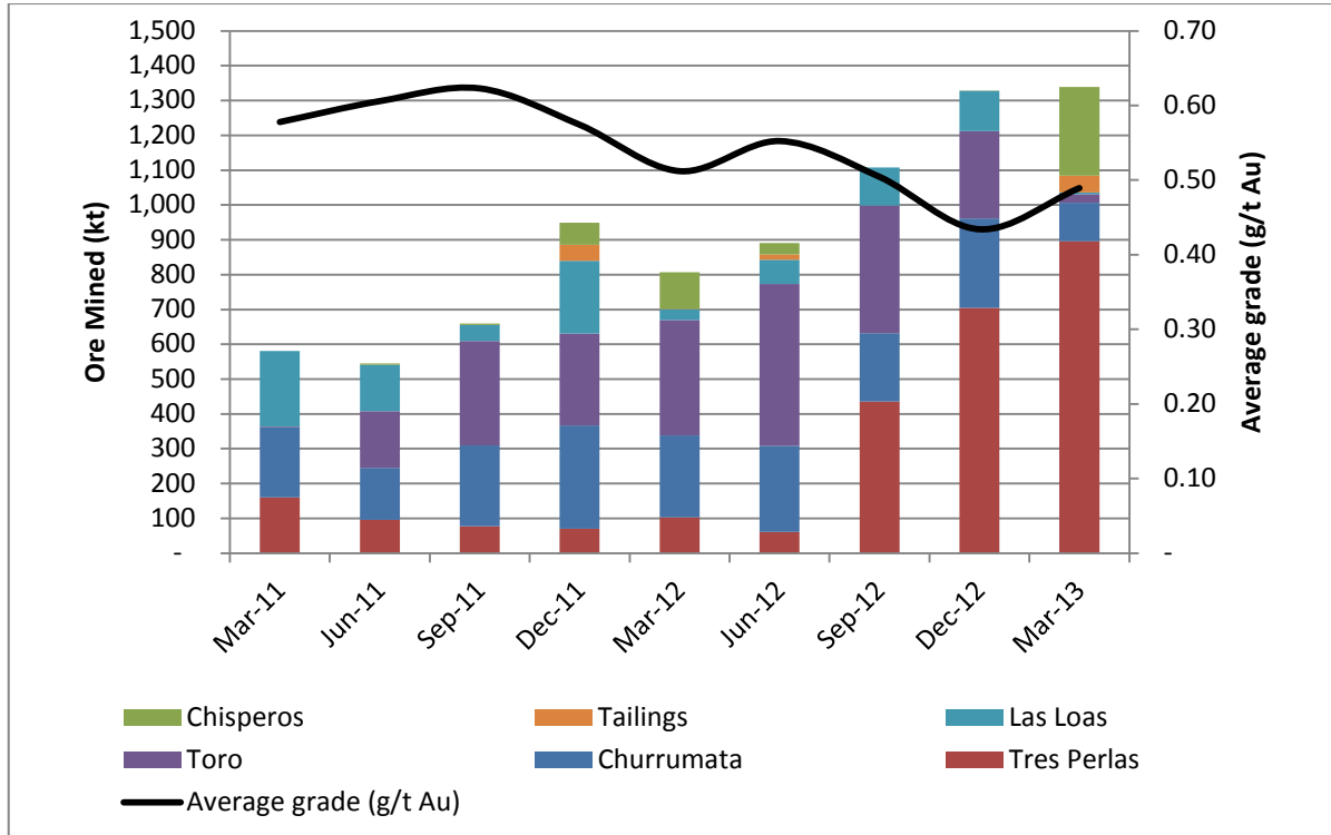
Figure 5– Ore Mined by Pit and Quarter
