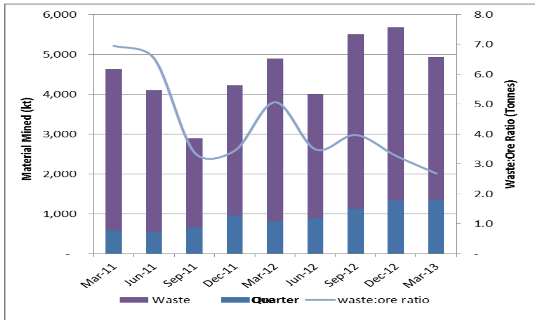
Figure 4 – Material Mined and Waste to Ore Ratio by Quarter
