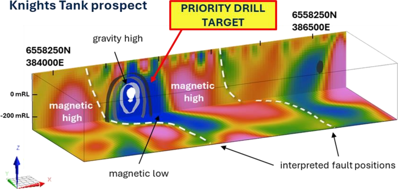
Figure 7 – Isometric geophysical block model mages showing ground gravity 3D density contrast Iso-Shells (up to 0.14 g/cc) on magnetic 3D inversion ( SI \times 10^{-6} ) model. Geophysical and structural features annotated, and priority drill target areas highlighted.
