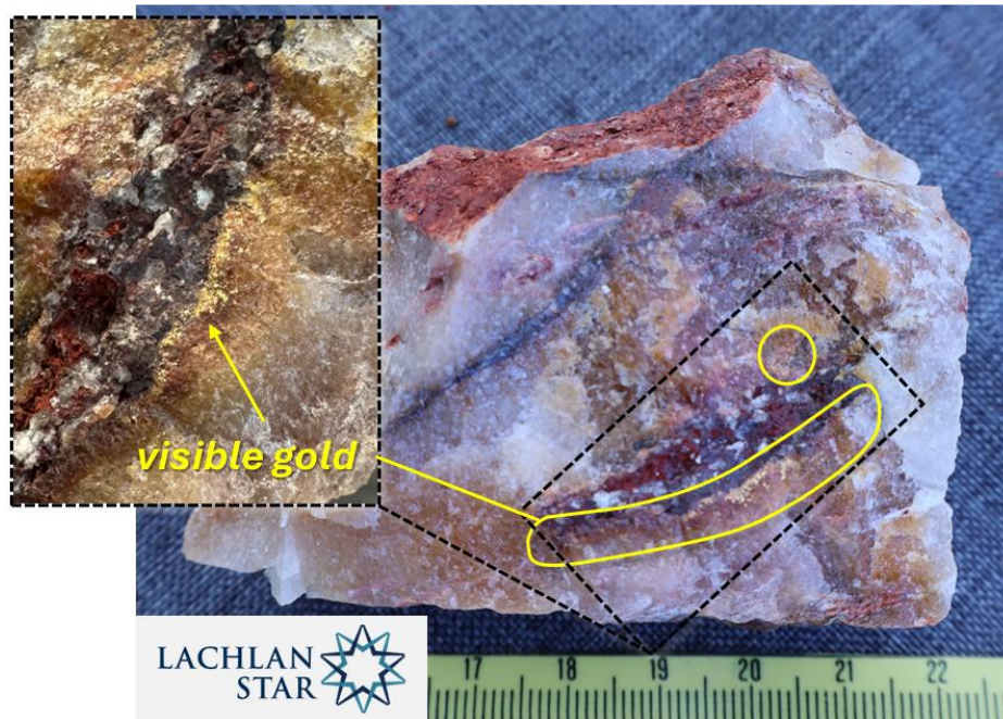
Figure 5b: The rock chip sample presented in Figure 5b shows semi-massive quartz vein material from the west-east crosslink quartz reef in Trial Pit, with weathered and oxidised fracture surfaces containing iron oxides (hematite, goethite and limonite). Internally the quartz vein contains clasts of iron oxides (hematite and goethite) and silica fragments (2-3mm in size) with fine (<0.5mm in size) gold occurring as an aggregate along the margins of the iron oxide clast as well as disseminations throughout.
