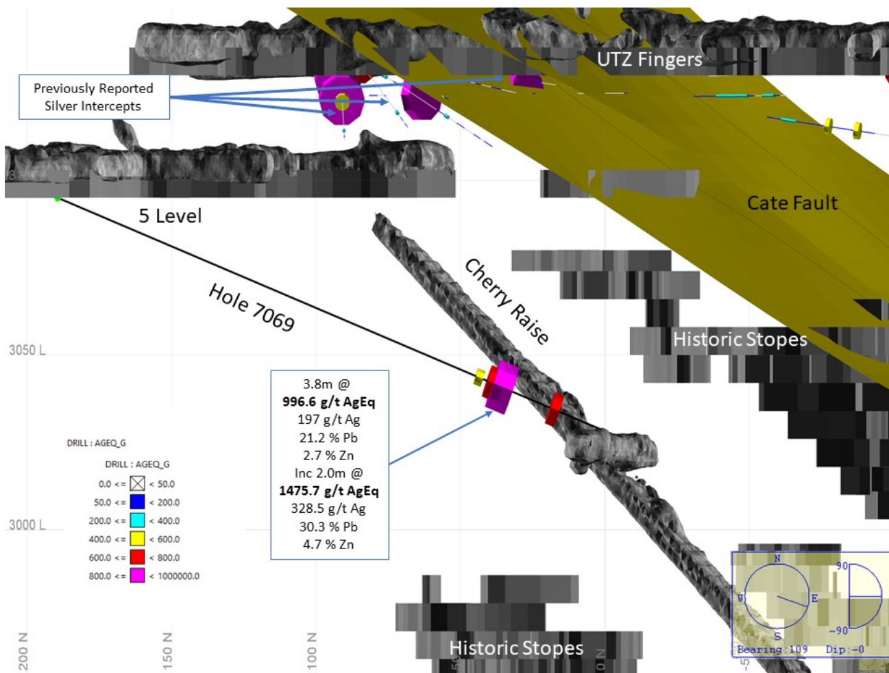
Figure 2: Cross section of hole 7069
