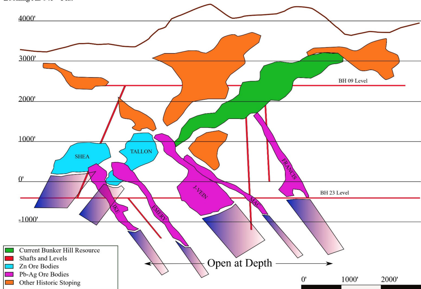
Image 2: Idealized long section of historic Bunker Hill workings and estimated 2021 PEA resource boundary
