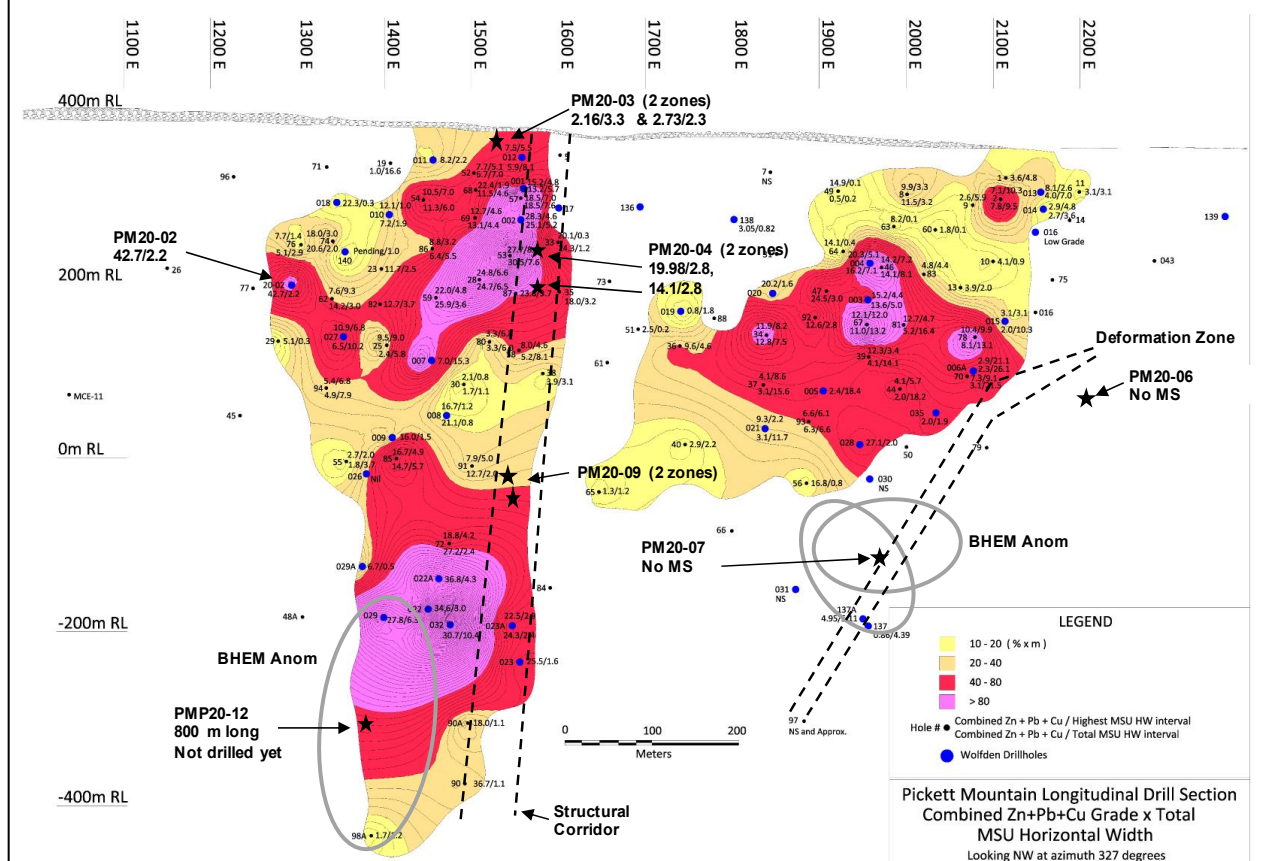
Figure 2. Vertical Longitudinal Section of West and East Lenses
