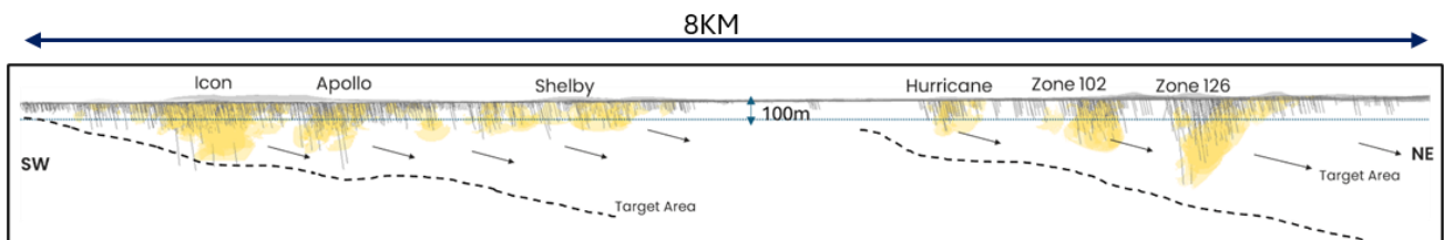
Figure 4 Long section, looking north highlighting strategic exploration search space at Glenburgh, with all known mineralisation open at depth
