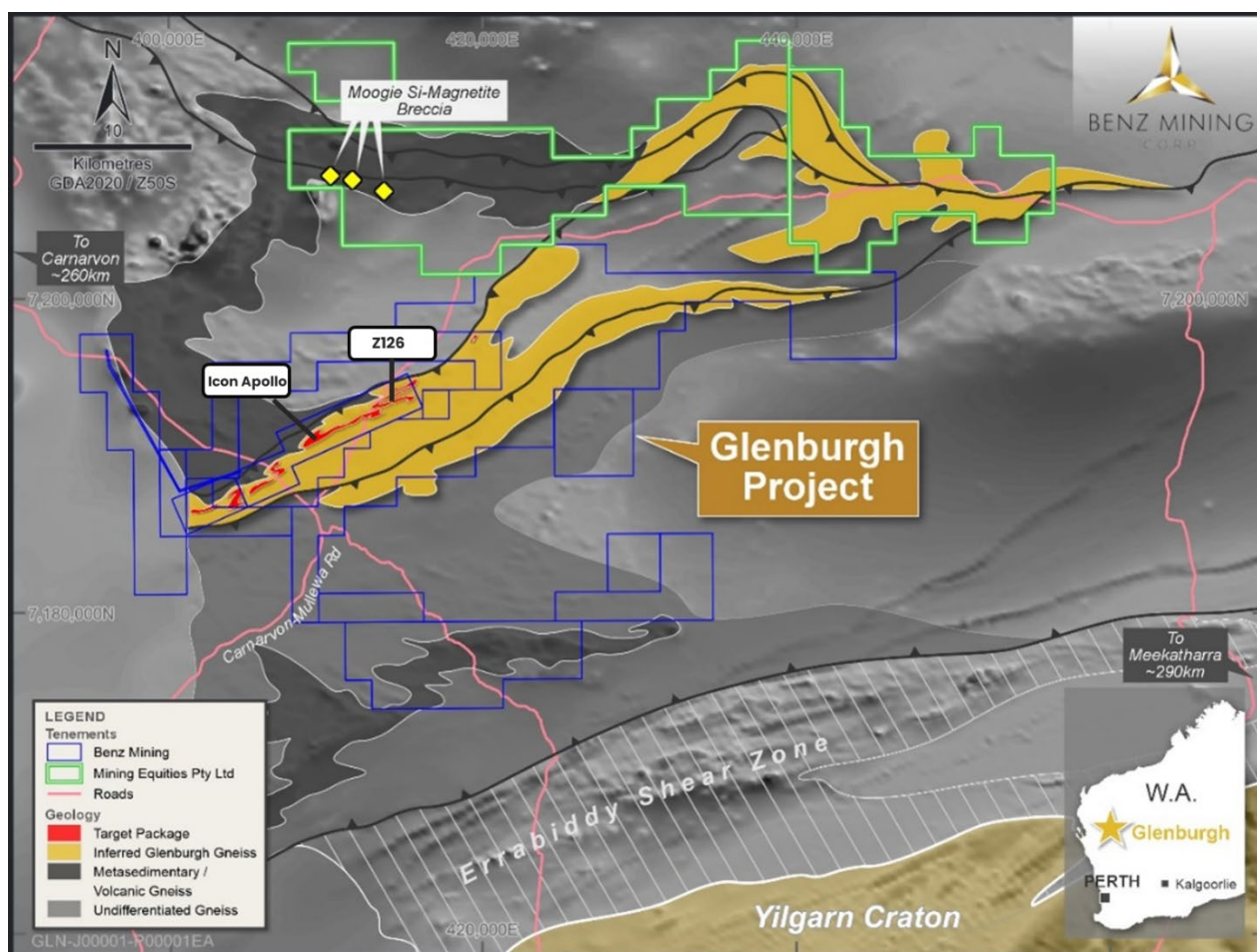
Figure 2 Glenburgh Project Geology overview.
