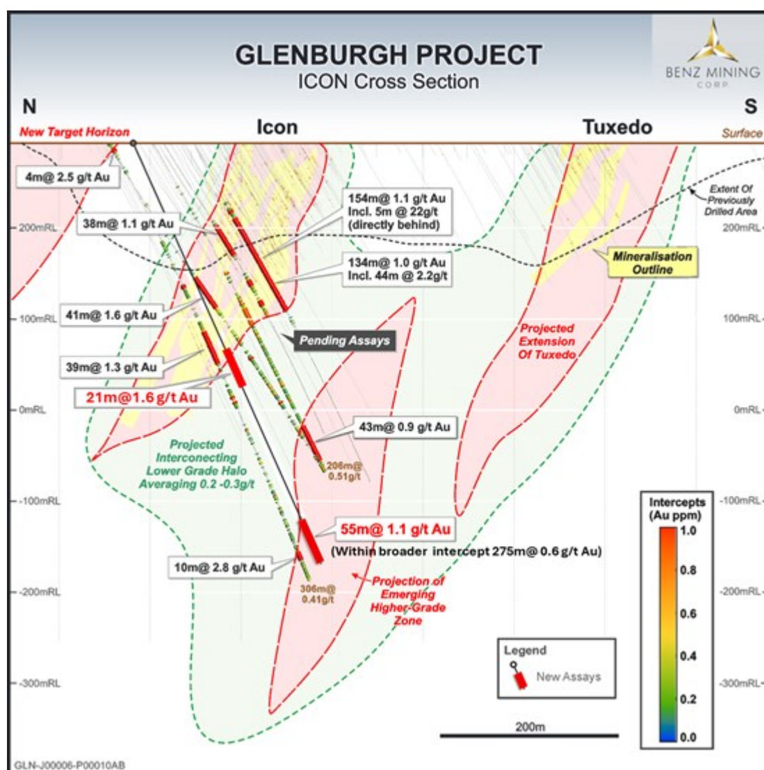
Figure 2: Cross section at Icon with viewing window (~300m) looking east along 409650 Easting. Current drill holes extend mineralisation under previously intercepted mineralisation conducted by historical drilling. Previous holes reported in announcement dated 4 August 2025.
