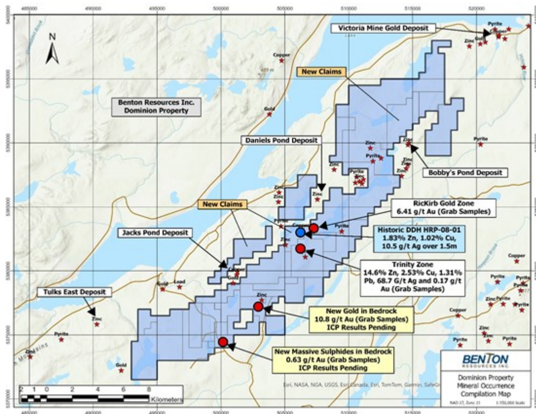
Figure 1: Regional Compilation and Mineral Occurrence Map
