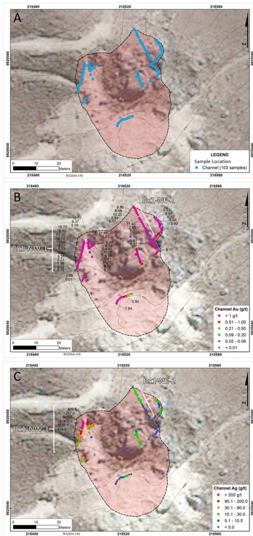
Figure 1 - Maps for Bx1 showing A) channel sample locations, B) gold distribution (samples >5.00 g/t Au labeled), and C) silver distribution (samples >200.0 g/t Ag labeled). Dashed outline shows approximate limit of breccia outcrop (red shaded area). Two longer continuous channel samples highlighted (Bx1-NW-1 and Bx1-NE-1).
