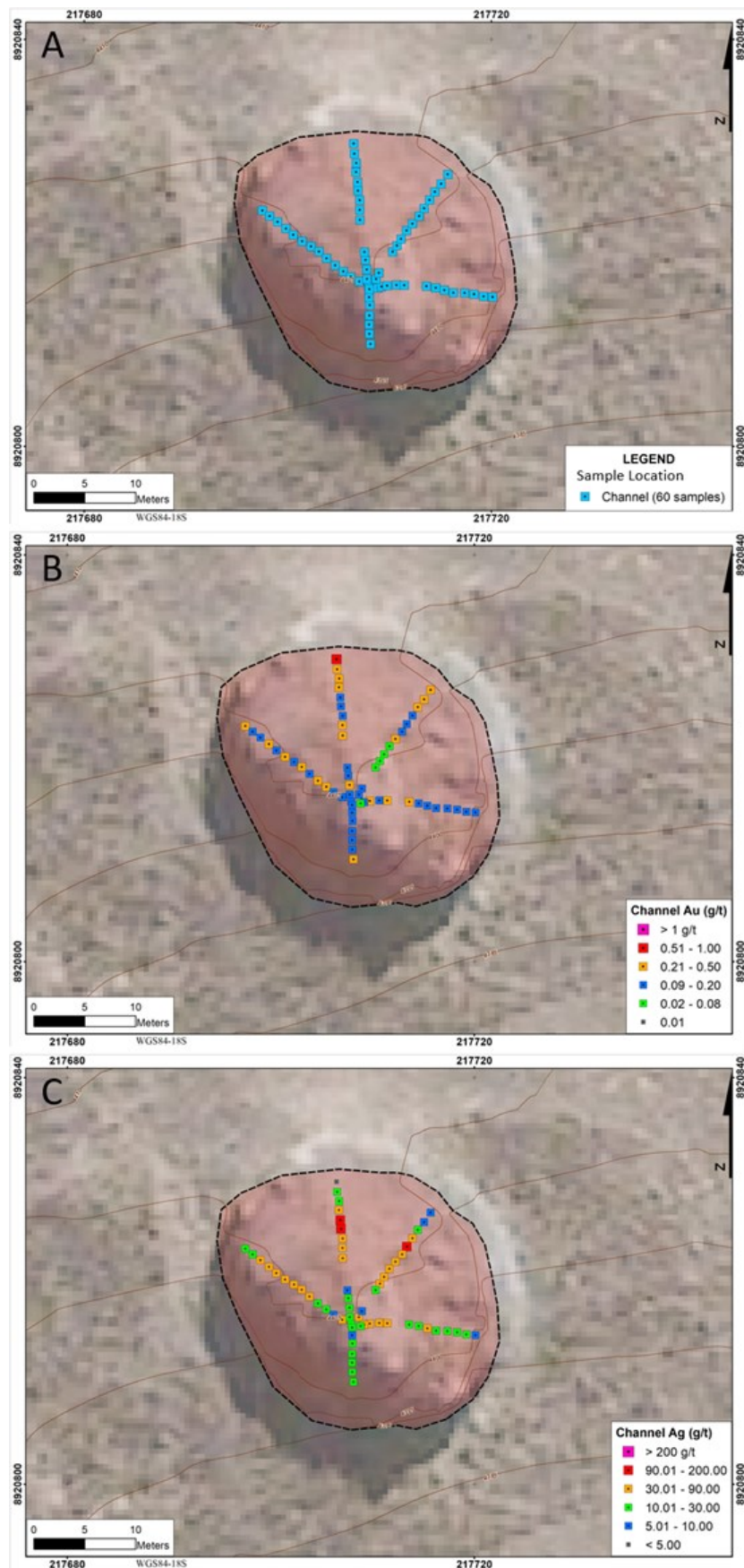
Figure 2 - Maps for Bx6 showing A) channel sample locations, B) gold distribution, and C) silver distribution. Dashed outline shows approximate limit of breccia outcrop (red shaded area).
