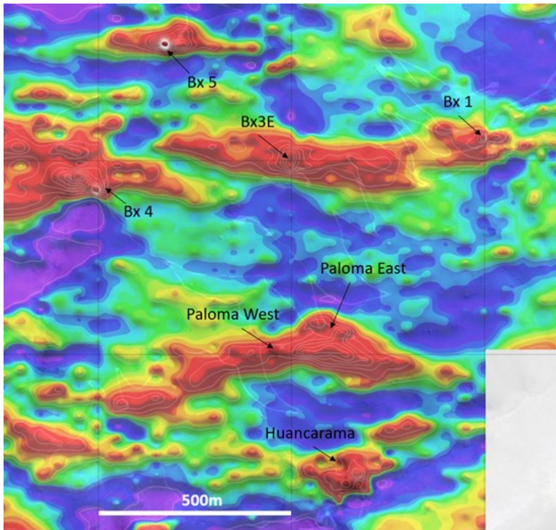
Figure 4 - Gradient-array IP map for the north-central Soledad project area showing metal factor - a scaled ratio of the measured IP and resistivity responses. Warm colors depict areas where the rocks are conductive and chargeable. Long linear trends are interpreted to be structures and are considered highly prospective for hosting mineralized breccia pipes.
