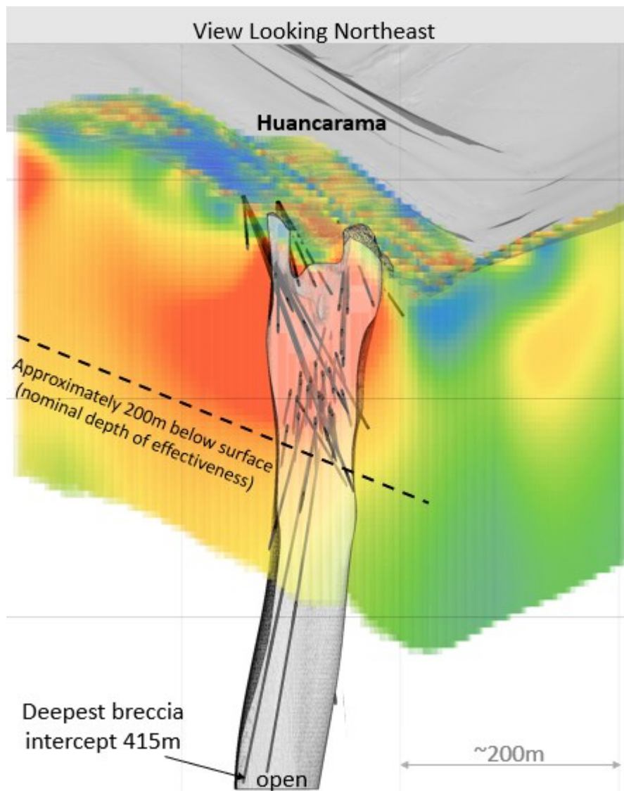
Figure 5 - Isometric view of offset IP/Resistivity inversion model results showing metal factor - a scaled ratio of the measured IP and resistivity responses. Warm colors depict areas where the rocks are conductive and chargeable. Note correlation between strong metal factor response (red) and the Huancarama breccia pipe confirmed in drilling.
