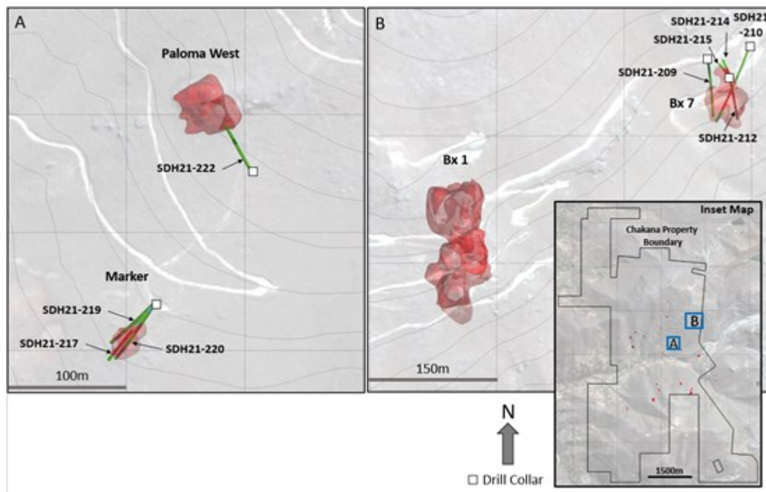
Figure 2 - Maps showing drill holes reported in this release, and modeled breccia pipes (light red shapes) based on all drill holes. Light gray contours are at 25m intervals. Blue rectangles in the inset map show the area of the two plan maps within the overall Chakana property.
