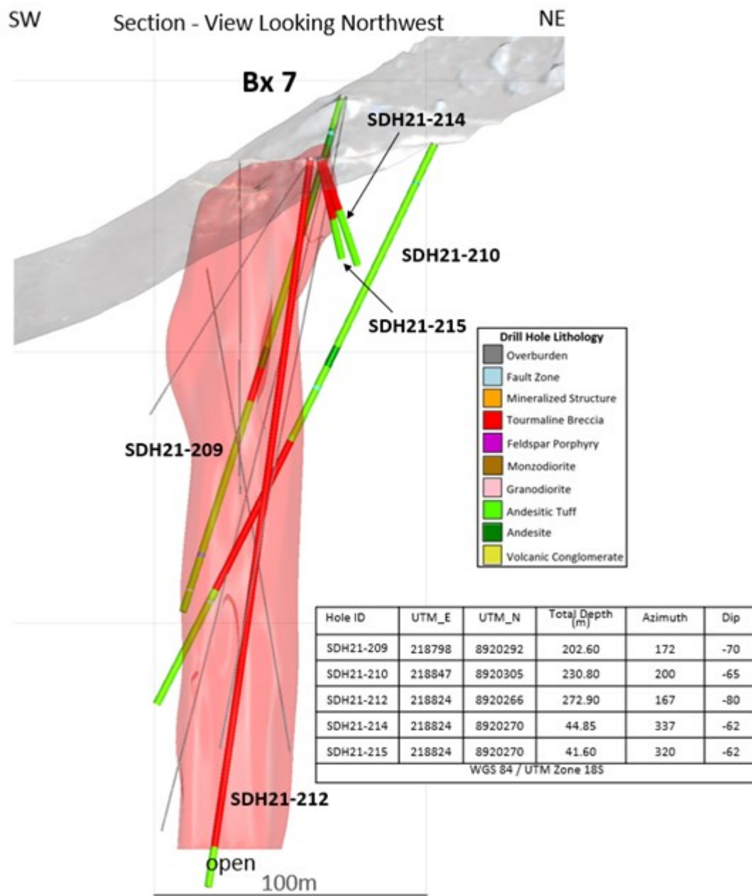
Figure 3 - 3D sectional view of Bx 7 looking northwest. Light red 3D shape shows breccia pipe geometry based on all drill holes. Previous holes drilled shown in grey.
