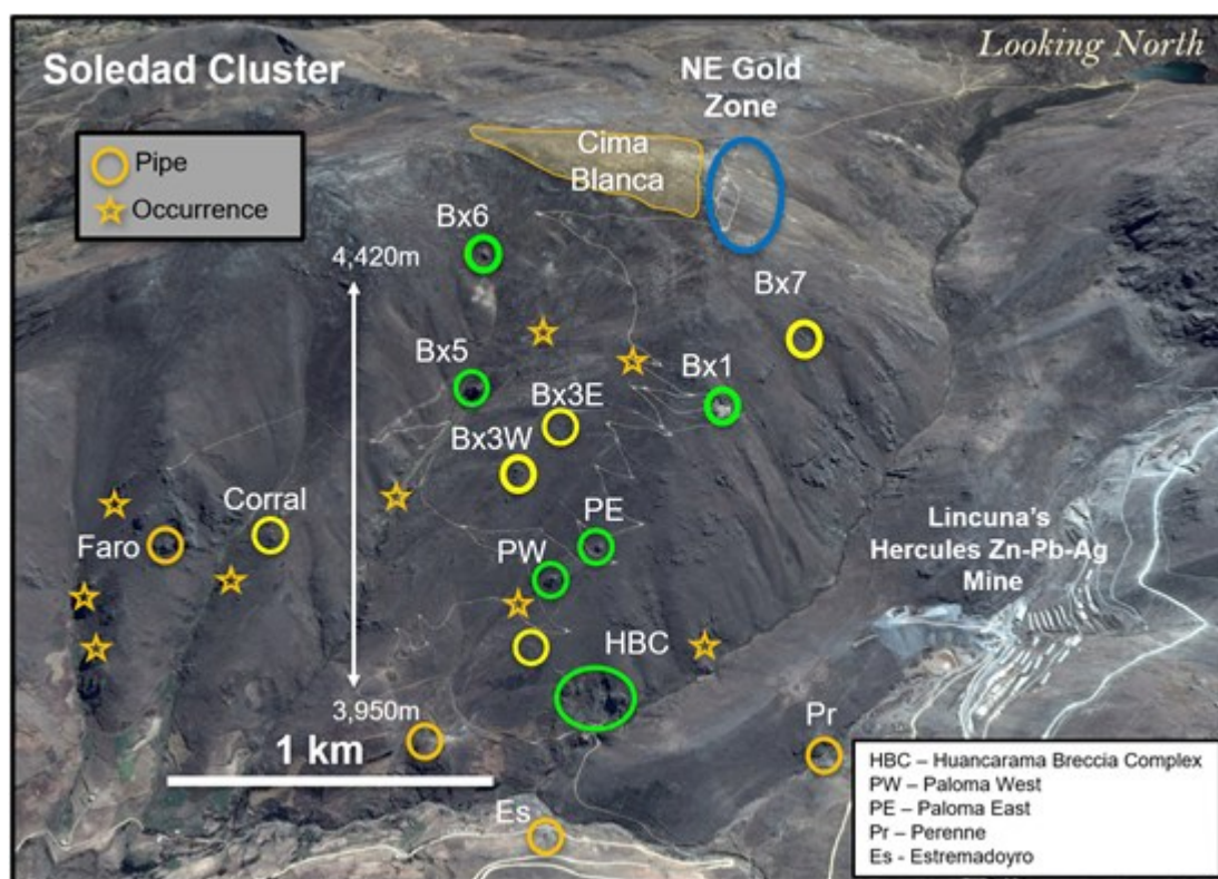
Figure 1 - View looking north showing outcropping breccia pipes and occurrences within the northern Soledad cluster. Pipes that have initial resource drilling completed shown in green. Breccia pipes shown in yellow have had exploration drilling completed. Other pipes and occurrences remain to be tested by drilling. Additional breccia pipes occur on the south half of the property and are not shown here.
