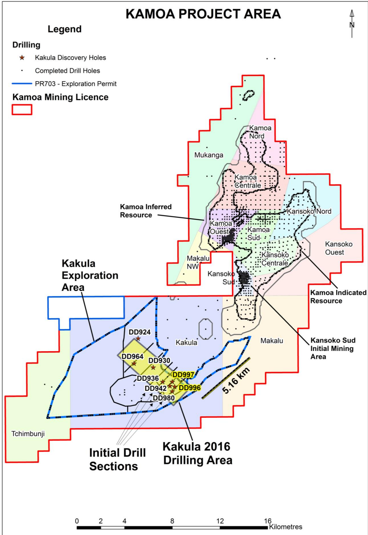
Figure 1: Kamoia plan map showing Kakula exploration area, discovery drill holes and 2016 drilling area.
