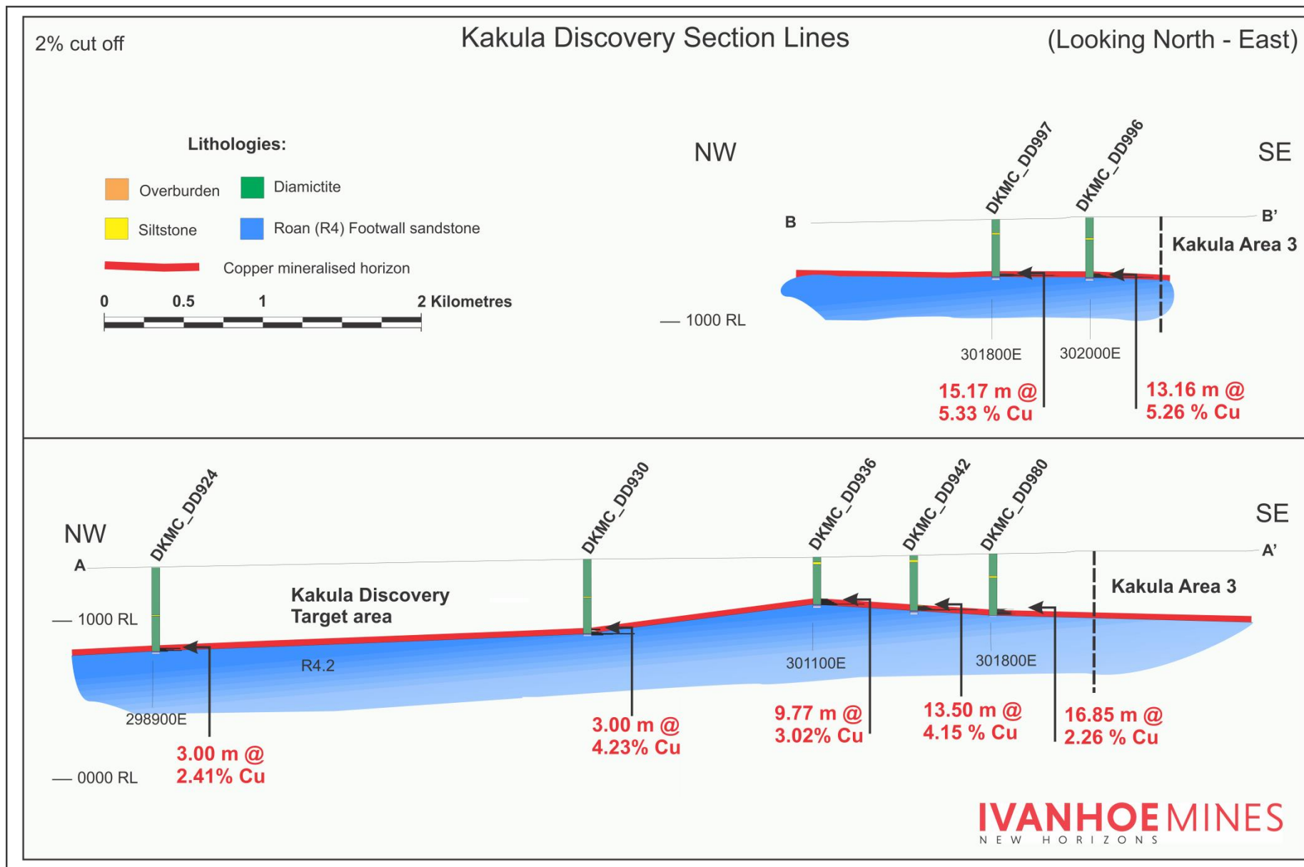
Figure 3: Sections across the Kakula Discovery Area
