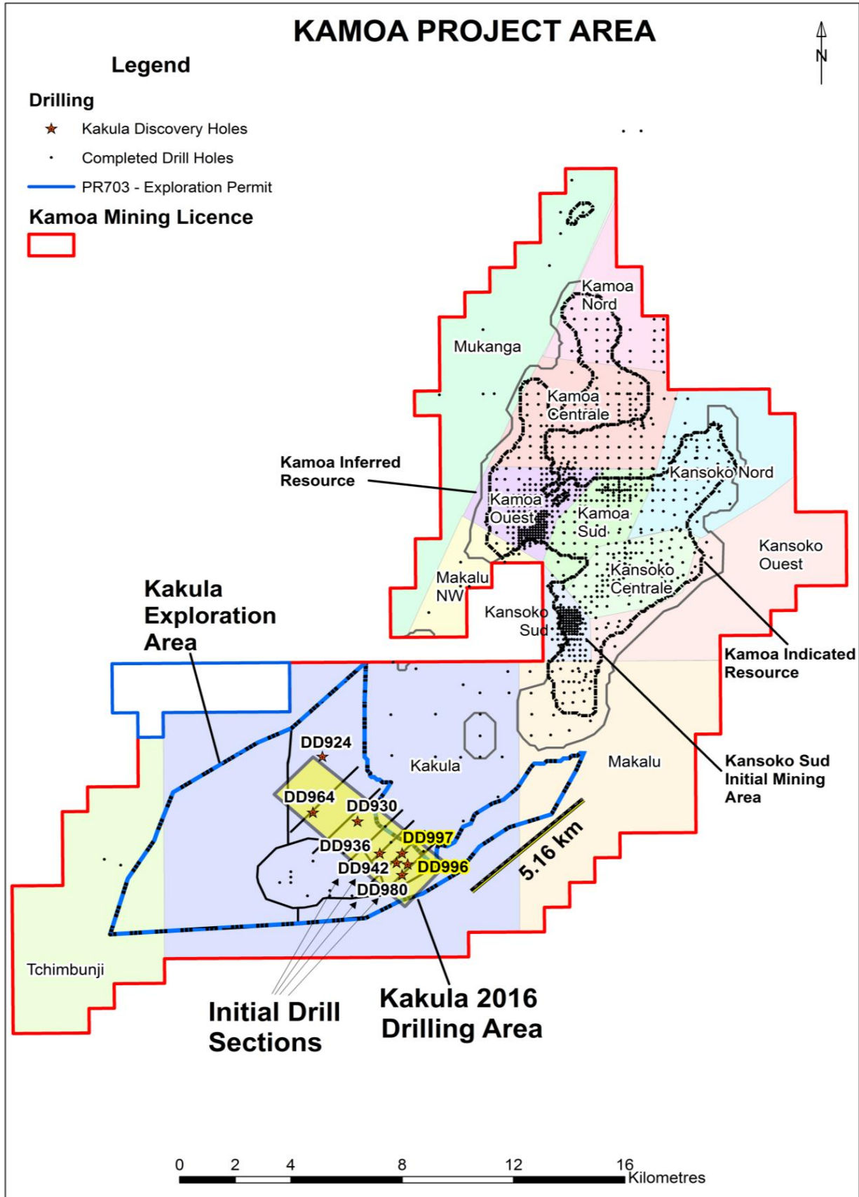
Figure 4: Kamoa Project area map showing the Kakula exploration area.
