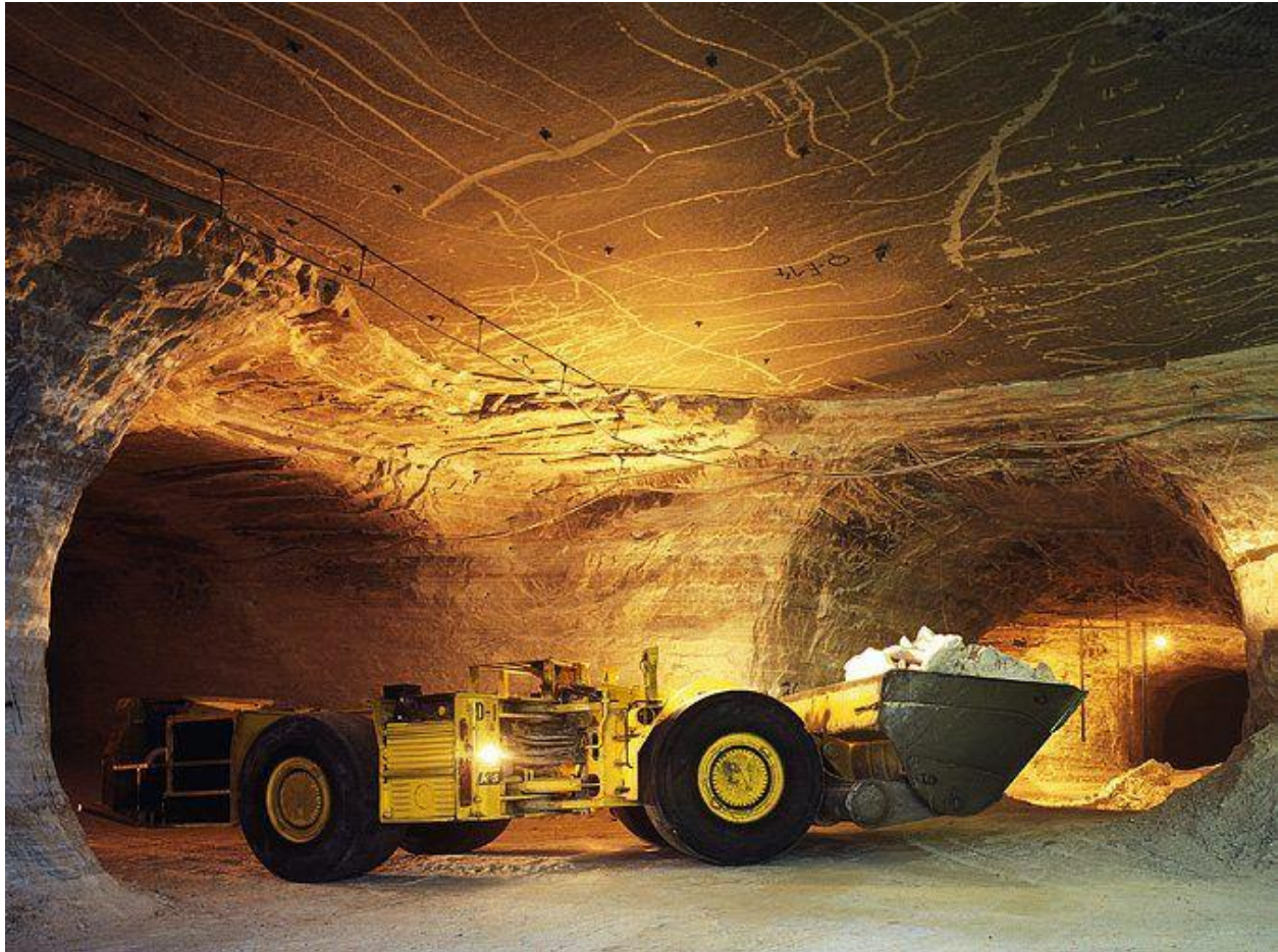
Figure 6. A 17-tonne loader in operation at an approximate six-metre-high, underground room-and-pillar potash mine in Canada (for illustration purposes only). Kamo'a's Kansoko Sud and Kakula deposits are expected to use similar underground mining methods and equipment.
