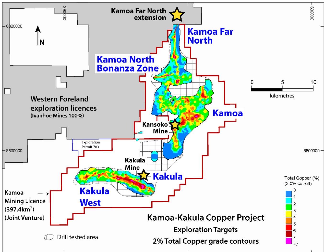
Figure 2: Kamo-Kakula mining licence, showing the Kamo North Bonanza and Kamo Far North zones, the new Kamo Far North extension discovery on Ivanhoe's 100%-owned exploration licences, and the planned mines at Kakula and Kansoko.
