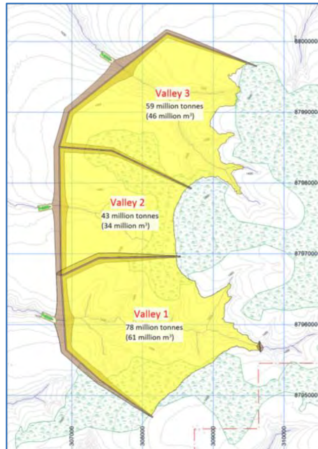
Figure 20.4 Kakula TSF layout for 180 million tonnes
