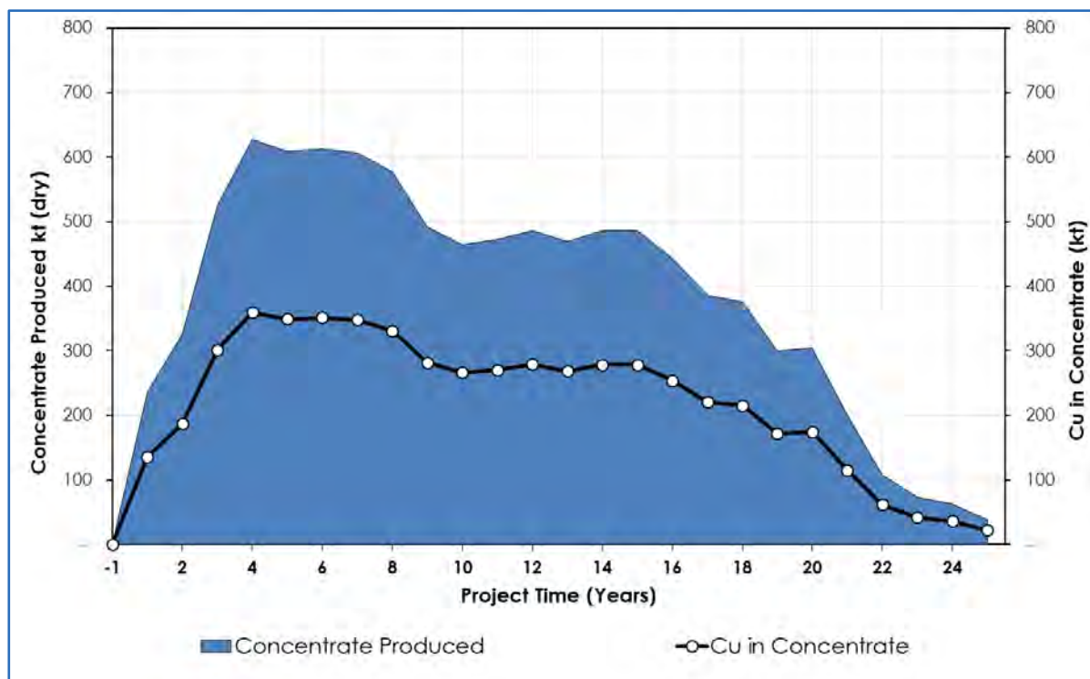
Figure 1.9 Kakula 2019 PFS Concentrate and Metal Production
