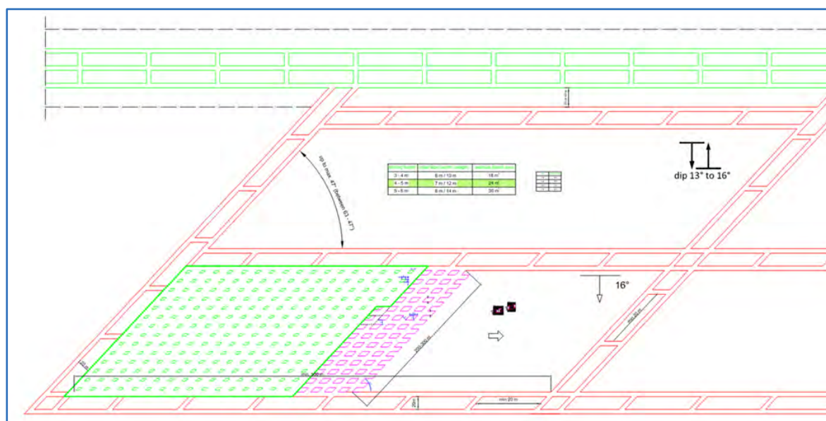
Figure 16.11 Controlled Convergence Room-and-Pillar Mining Method and Pillar Geometry for a Deposit with Dip Angle of 13 to 16°
