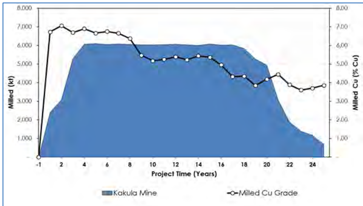
Figure 1.8 Kakula 2019 PFS Process Production
