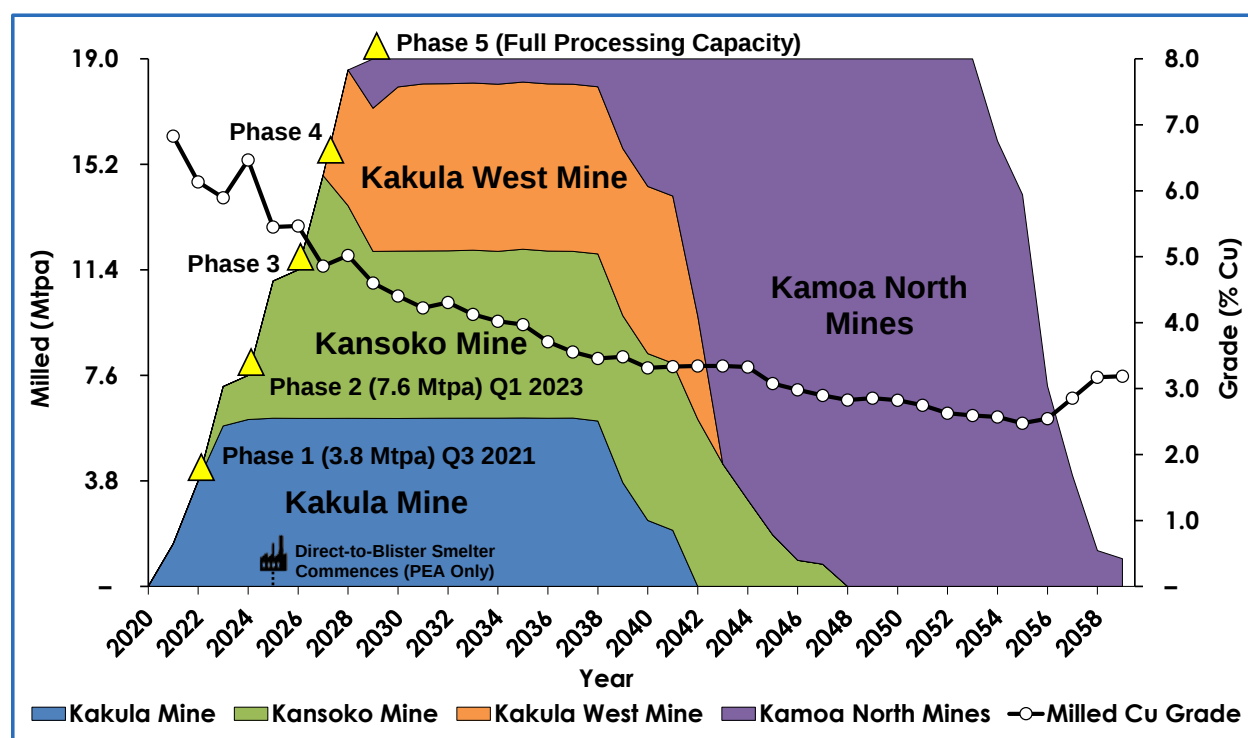
Figure 1. Kamoia-Kakula 19-Mtpa PEA long-term development plan, which would position Kamoia-Kakula as the world's second largest copper mining complex, with peak annual copper production of more than 800,000 tonnes.
