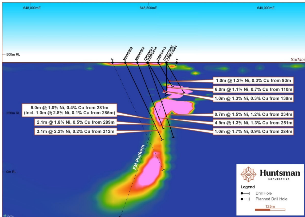
Figure 2: Cross section of Tulloch zone with modelled EM conductor and historical drilling.
