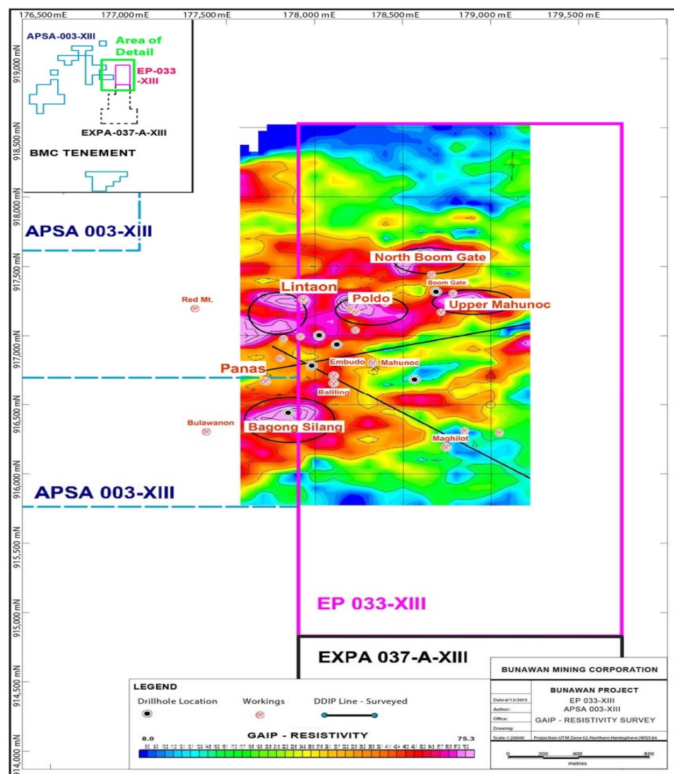
Figure 2 - Bunawan GAIP Resistivity Survey
