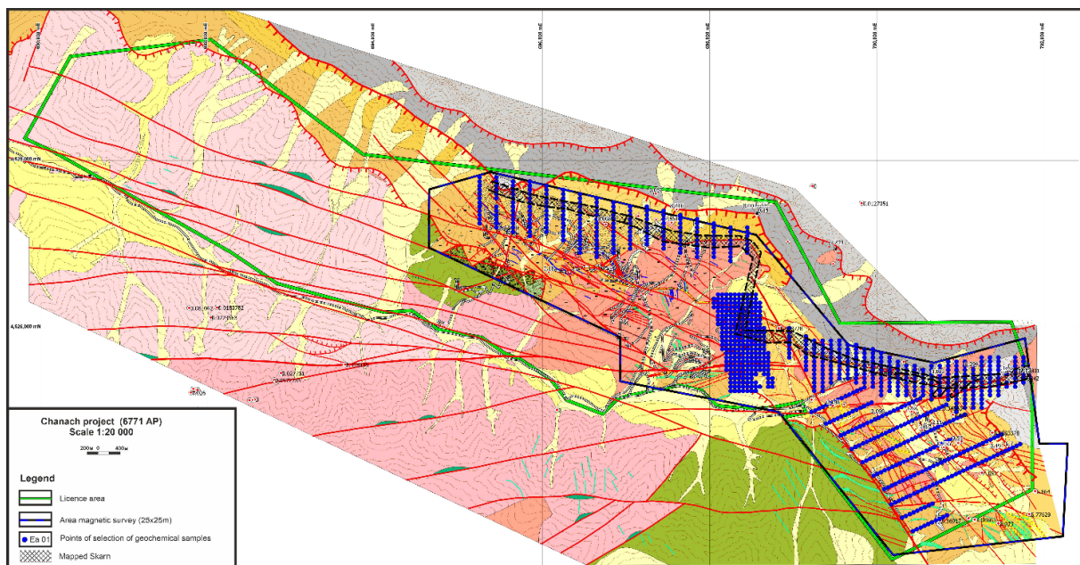
Figure 3: Tenement Map showing area of 2023 Field Season Geochemical Samples and Magnetic Survey
