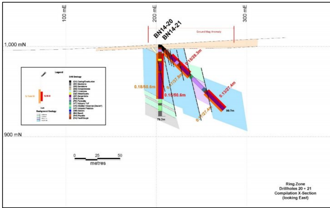
Figure 45: Ring Zone: X-Section 3 (Holes 14-20 and 14-21)
