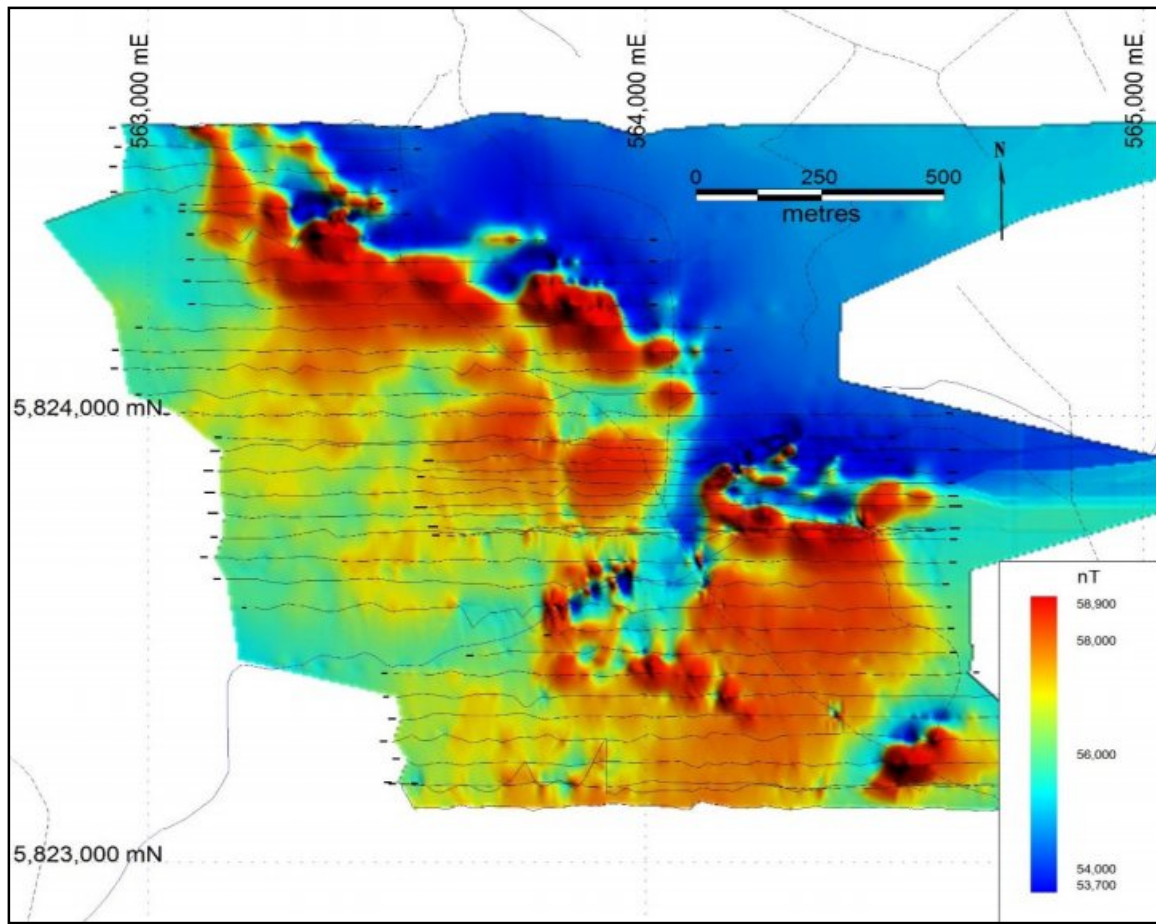
Figure 26: Skelton Grid Ground Magnetism (TF)
