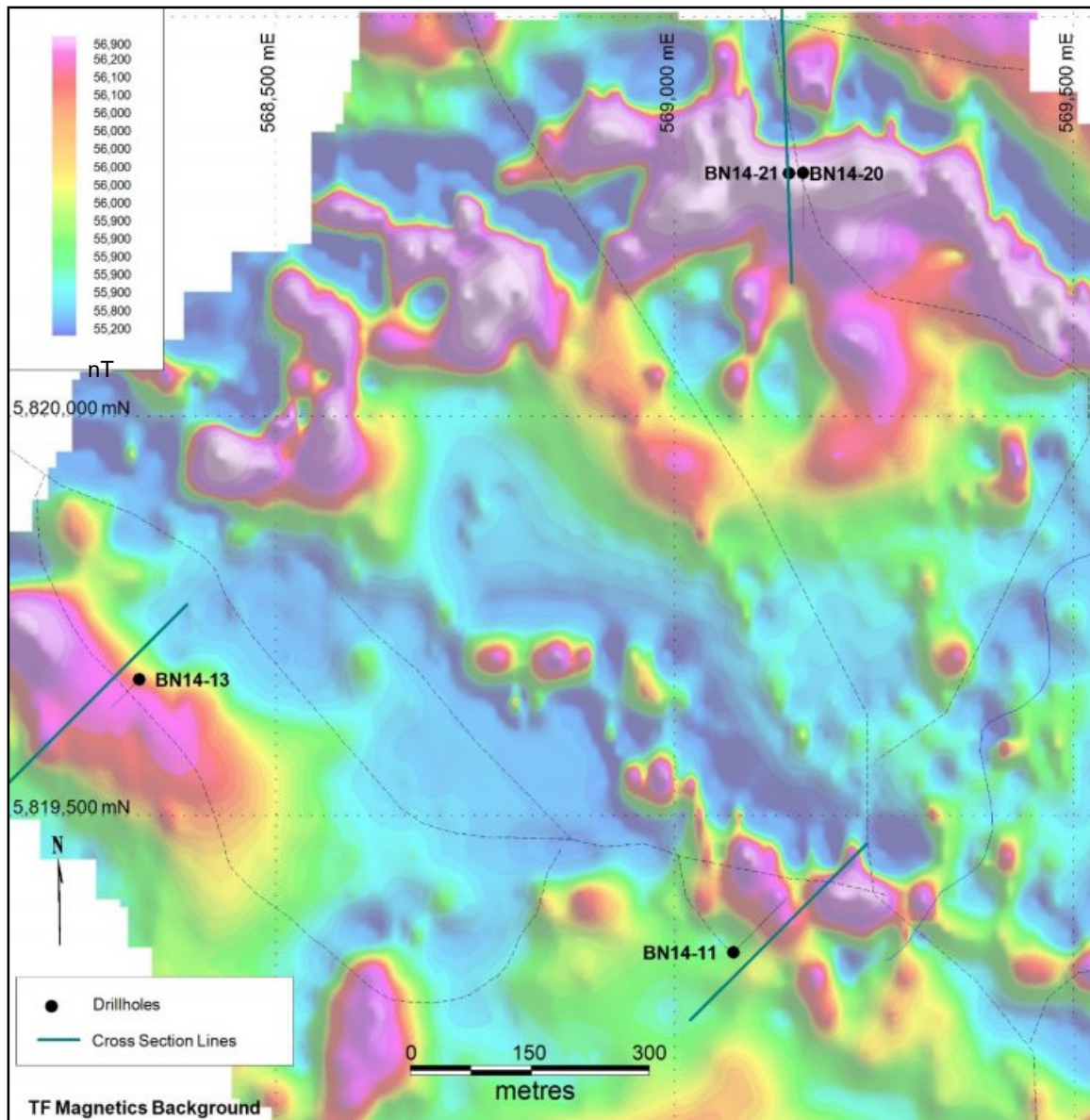
Figure 42: Ring Zone Drill Locations (Total Field Magnetics Background)
