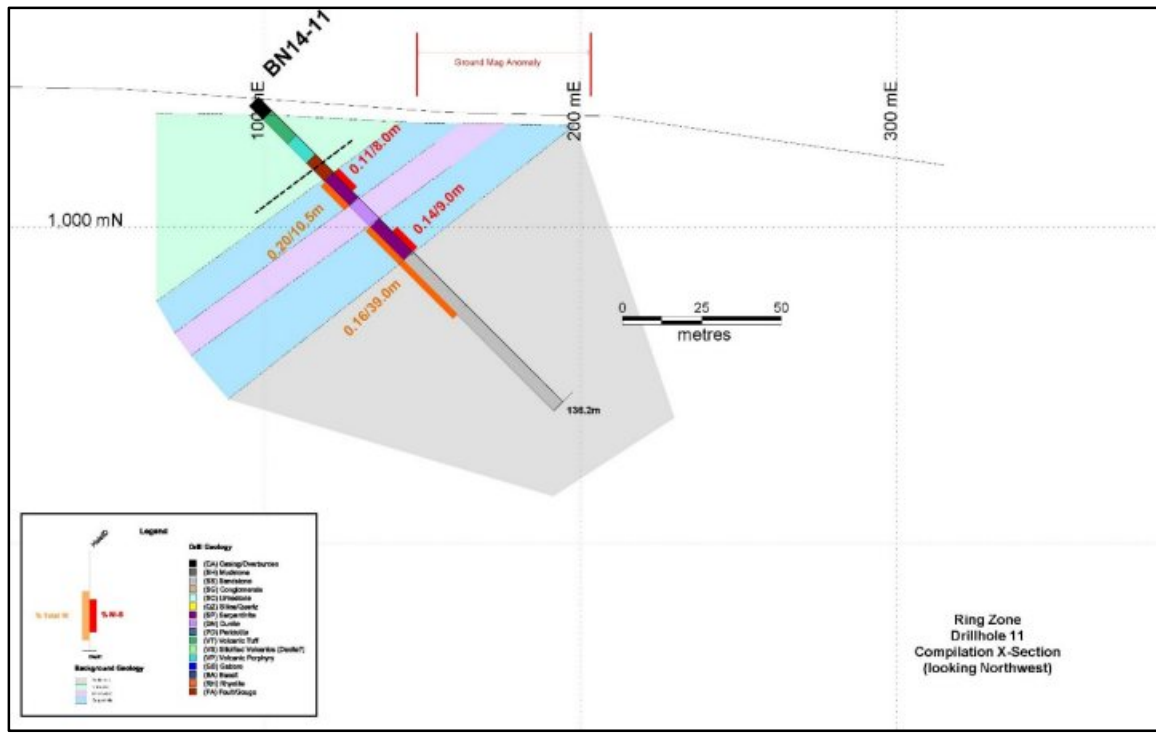
Figure 43: Ring Zone: X-Section 1 (Hole 14-11)
