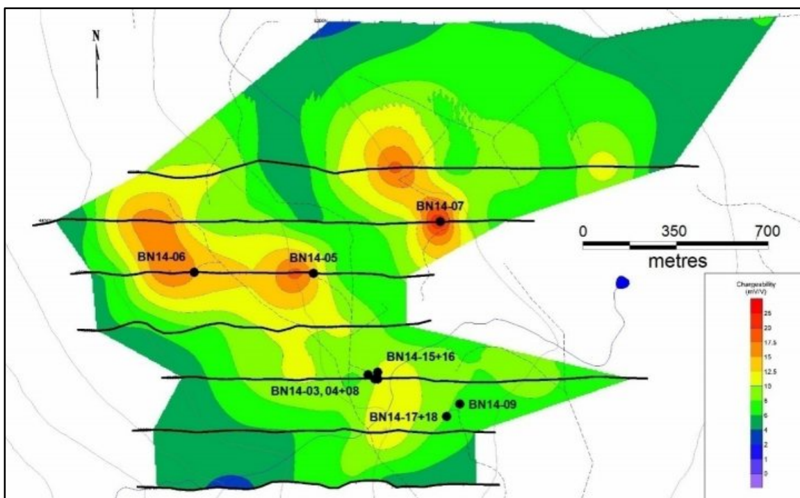
Figure 31: Skelton Zone IP Chargeability Compilation (Inverted Plan Slice at 100m Depth)
