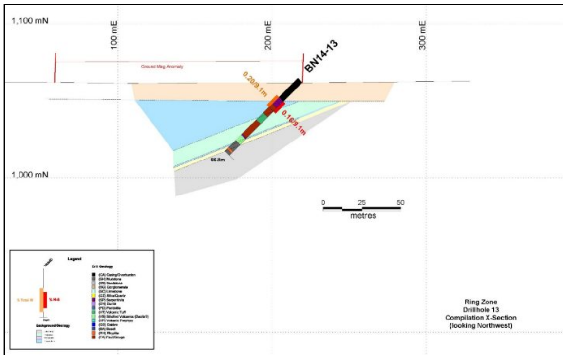
Figure 44: Ring Zone: X-Section 2 (Hole 14-13)
