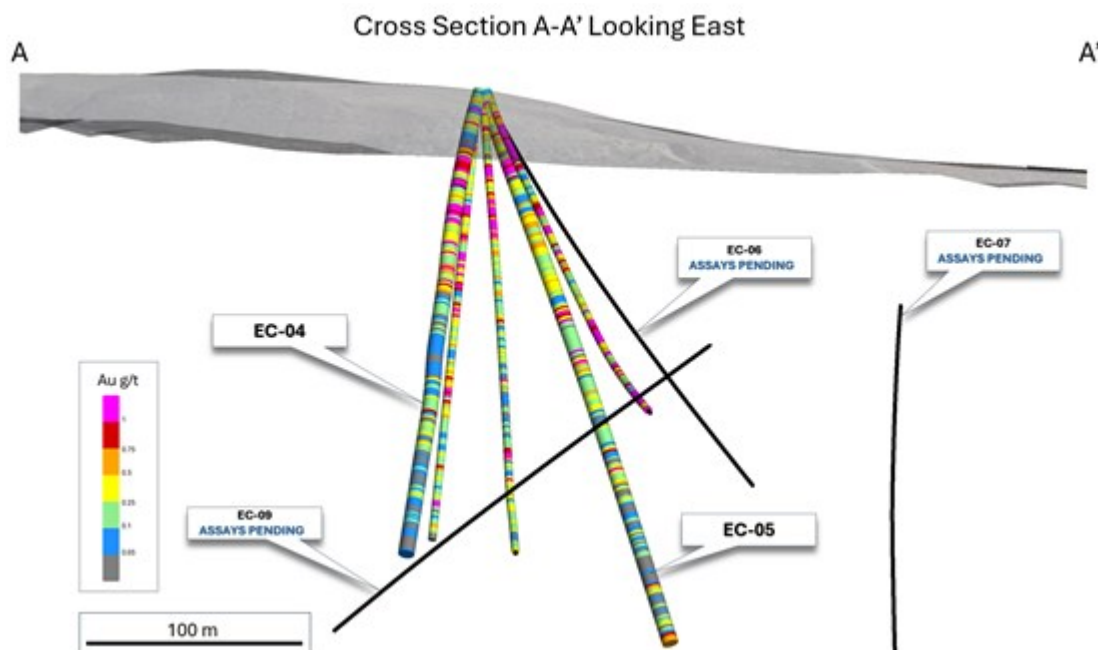
Figure 2. Cross Section Showing Herman Drill Hole Locations and Gold Assays.
