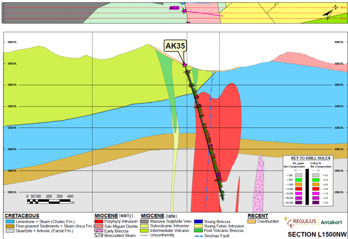
Figure 3-Section L1500NW-Hole AK-19-035
