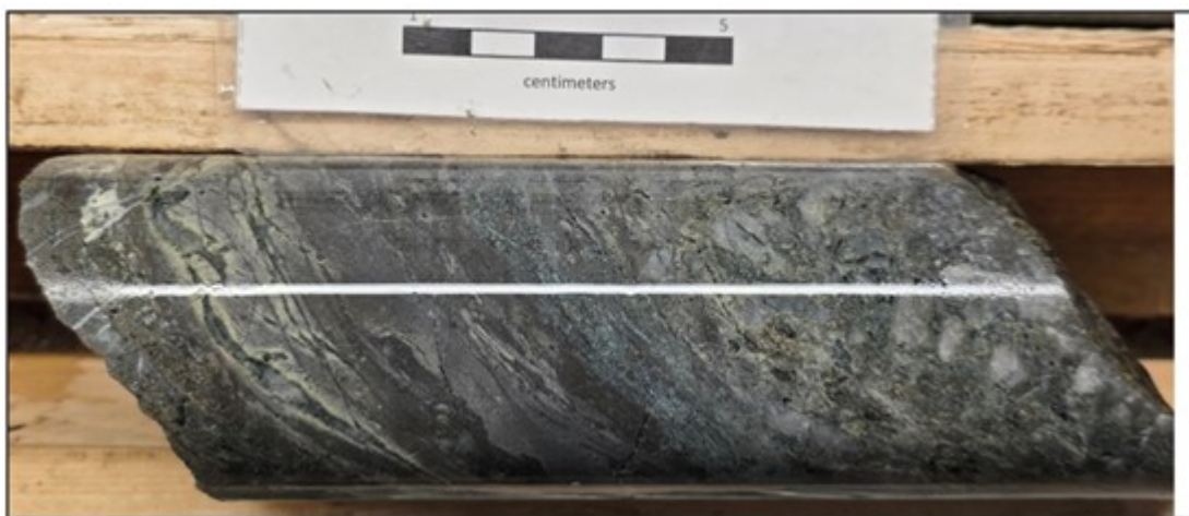
Photo 5. Banded quartz vein with disseminated and banded sulphides (Alt-25-013, 36 m depth - 8.2 g/t Au over 0.83 m, from 35.29 m depth).
