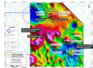
El Cobre Project Exploration Targets
