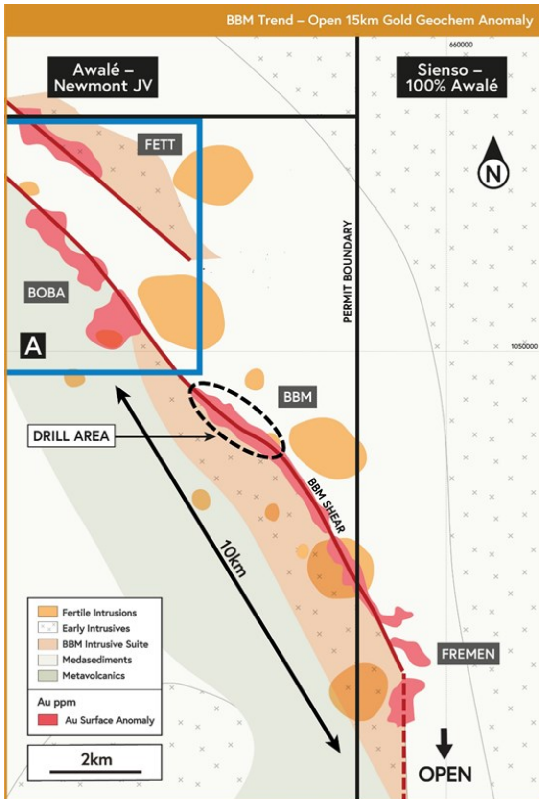
Figure 3: The 15km-long BBM shear - A 15km trend with Fremen to the southeast, BBM, and Boba and Fett targets to the north.
