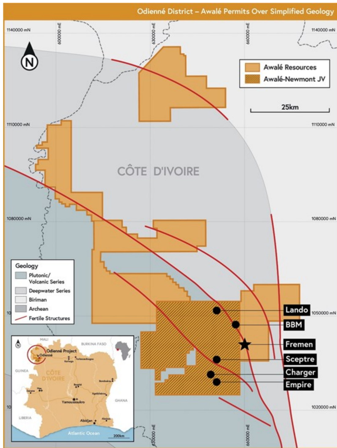
Figure 1: The Odienné Project - 2,462 square kilometres, showing targets for the project area.
