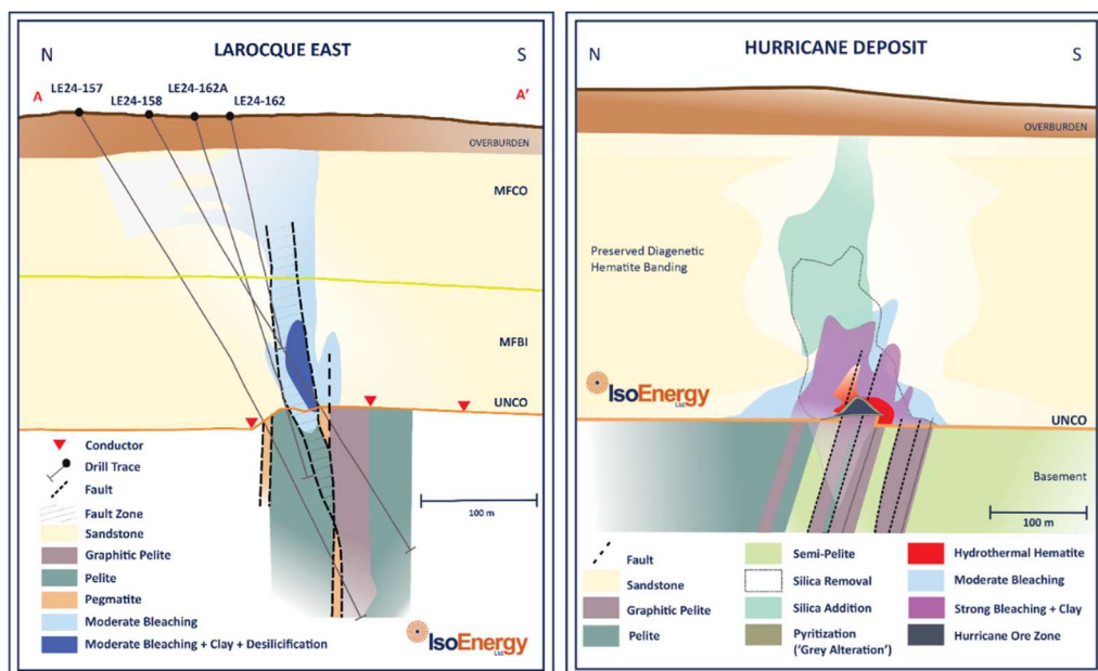
Figure 2 – Larocque East Target Area A geological cross section looking east (left). The section is drawn through the eastern end of Area A and the location of the section is shown on Figure 1. Features shown including graphitic pelite basement rocks, subvertical faults, relief on the unconformity surface, and bleaching, clay alteration and desilicification are also comparable and present at the Hurricane deposit (right) 2,100 m on strike to the west-southwest. Hurricane deposit cross section illustrating key characteristics of the alteration and basement structure and lithology associated with uranium mineralization (right).
